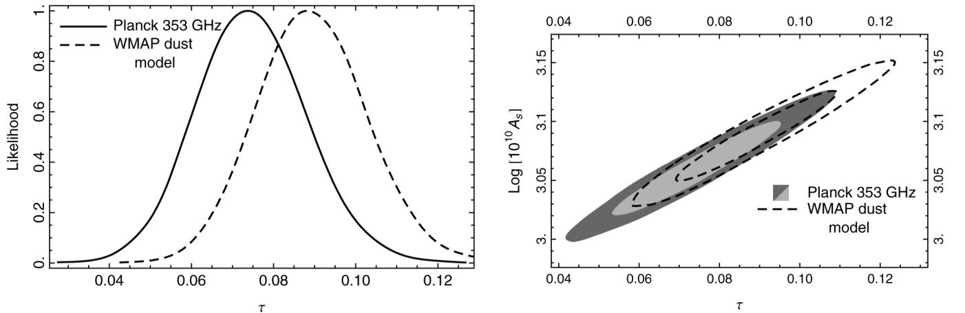
Fig. E.2. 1D ( left ) and 2D ( right ) posterior probability for \tau and the combination \tau - A_s , for two different Galactic dust templates. These are computed using dust template coefficients estimated with the WMAP “processing” mask. The difference in \tau is reduced to \sim 0.5\sigma if template coefficients are estimated outside the “P06” Galactic mask.
