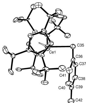
Fig. 2 ORTEP of \text{Cp}'_2\text{Ce}(4\text{-methylbenzyl}) , the half molecule of pentane in the unit cell is not shown. The non-hydrogen atoms are refined anisotropically and shown as 50% ellipsoids, the hydrogen atoms are not refined but they are placed in idealized positions and not shown. Selected distances ( \text{\AA} ) and angles (deg): \text{Ce-C}(\text{Cp}') = 2.86 \pm 0.08 , range 2.743(8) to 2.995(7), \text{Ce-Cp}'(\text{ring centroid}) = 2.60 , \text{Cp}'(\text{ring centroid})\text{-Ce-Cp}'(\text{ring centroid}) = 138.5 , \text{Ce-C}(35) = 2.576(7) , \text{Ce-C}(36) = 2.969(7) , \text{Ce-C}(37) = 3.933 , \text{Ce-C}(41) = 3.228 , \text{Ce-C}(35)\text{-C}(36) = 91.7(4^\circ) .
