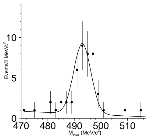
Figure 3: Signal events likelihood fit for the negative secondary beam.
