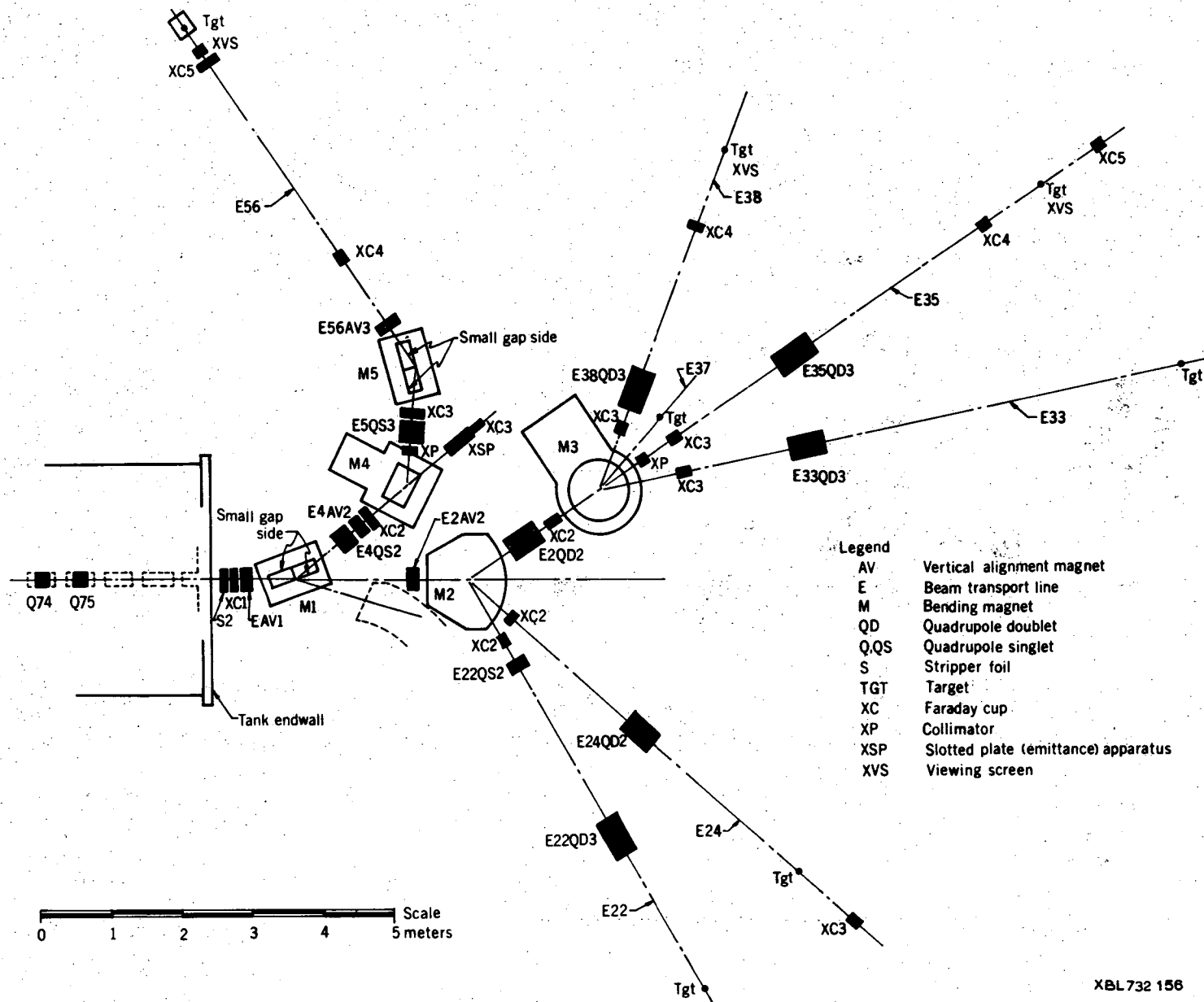
Figure 1. Plan of SuperHILAC experimental area beam lines as of February 1973.
