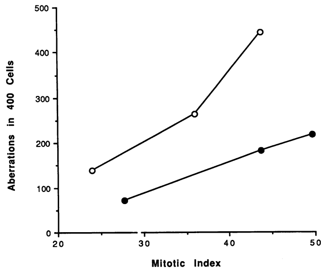
FIGURE 3. Decrease in yields of radon-induced chromatid deletions found in lymphocytes preexposed to 2 cGy of X-rays: independence of the mitotic index. (○) Cells exposed to radon alone; (●) cells exposed to X-rays plus radon. Data from Wolff et al. (14).
