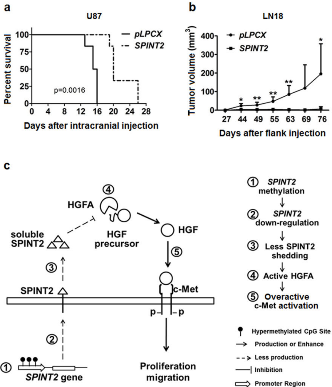
Fig. 5. SPINT2 overexpression diminishes tumor growth in vivo and prolonged survival of mice with intracranial transplantation.
