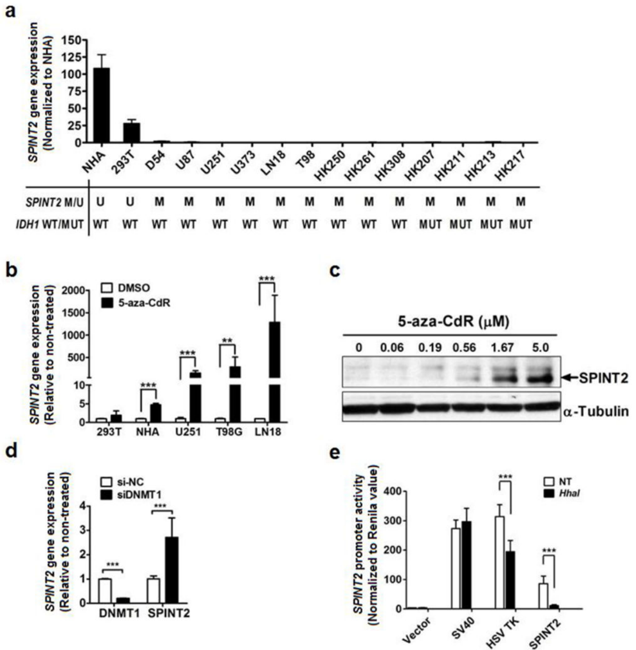
Fig. 2. SPINT2 expression is regulated by promoter methylation.
