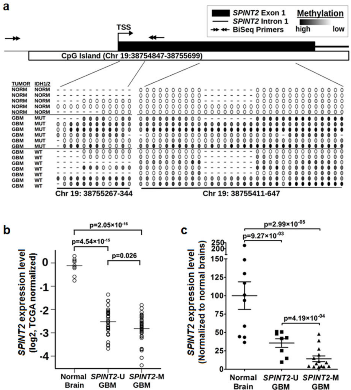
Fig. 1. SPINT2 is hypermethylated and downregulated in GBMs compared to normal brain tissues.
