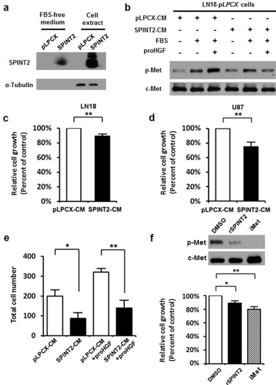
Fig. 4. SPINT2 protein diminishes c-Met activation, cell proliferation and invasion in LN18 cells. a. Starvation-derived conditioned medium of LN18- SPINT2 cells contained SPINT2 protein indicating shedding of soluble SPINT2 into medium by glioma cells (n=4, representative figure shown), b. Conditioned medium from LN18- SPINT2 cells suppressed c-Met activation in LN18- pLPCX cells. pLPCX-CM, serum-starvation-conditioned medium from LN18- pLPCX cells; SPINT2-CM, serum-starvation-conditioned medium from LN18- SPINT2 cells (n=3, representative figure shown). c. Conditioned medium from LN18- SPINT2 cells suppressed cell proliferation of LN18- pLPCX cells (n=3, mean \pm s.e.m). d.
