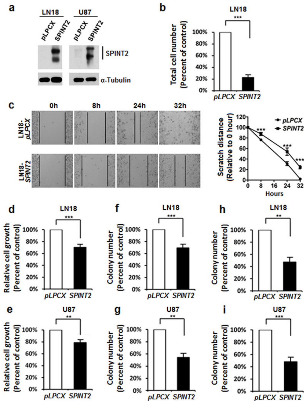
Fig. 3. SPINT2 overexpression blocks glioma cell invasion, migration and proliferation. a. Stable overexpression of SPINT2 in LN18 and U87 cell lines was achieved by retroviral infection and puromycin selection. b. SPINT2 overexpression reduced LN18 cell invasion in the Transwell migration assay ( n=6 , mean \pm s.e.m). c. SPINT2 overexpression inhibited the migration of LN18 cells in the wound healing assay ( n=6 , mean \pm s.e.m). d-e. SPINT2 overexpression reduced cell proliferation (MTT assay) in LN18 ( n=8 ) and U87 ( n=3 ) cells (mean \pm s.e.m). f-g. SPINT2 overexpression reduced colony formation in LN18 ( n=7 ) and U87 ( n=3 ) cells (mean \pm s.e.m). h-i. SPINT2 overexpression reduced anchorage-
