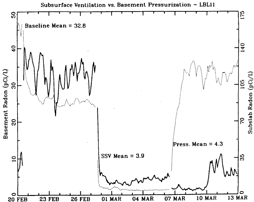
Figure 10. A comparison of the effectiveness of subsurface depressurization and basement pressurization in LBL11. Note that although indoor radon levels are low with both systems, the subslab soil gas radon concentrations (dotted line) remains high during basement pressurization. The average basement overpressure was approximately +1.2 Pa. The greater variability in radon levels during basement overpressurization result from the sensitivity of radon entry rates to basement pressures, which are, in turn sensitive to \Delta T and windspeed.
