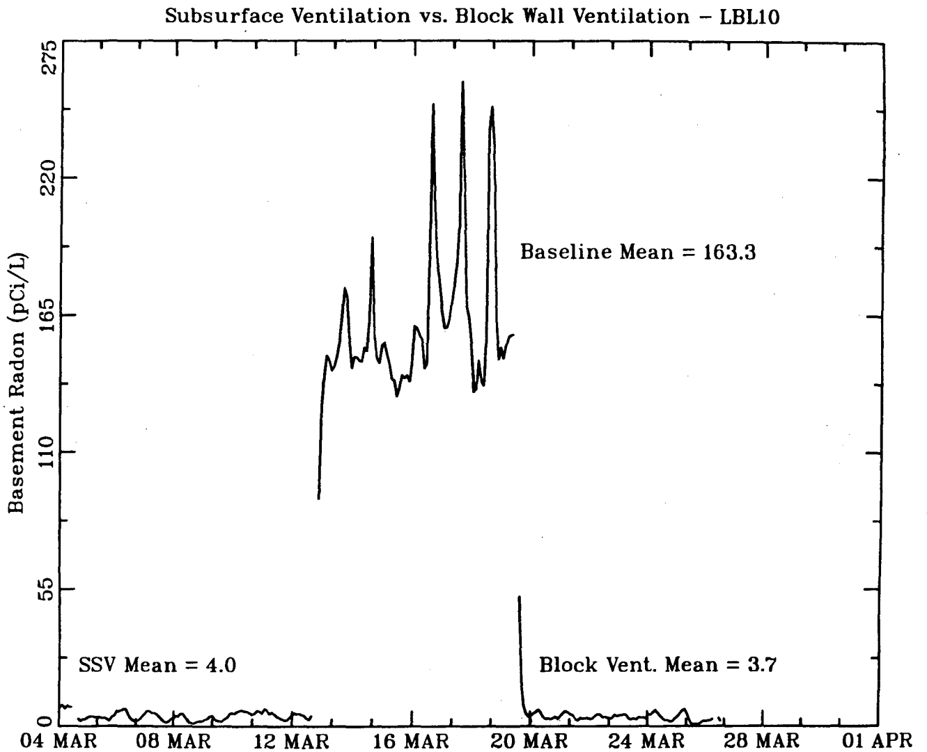
Figure 8. Comparison of block wall and SSD systems in house LBL10 during a four-week period. Performance of the two systems is almost identical.
