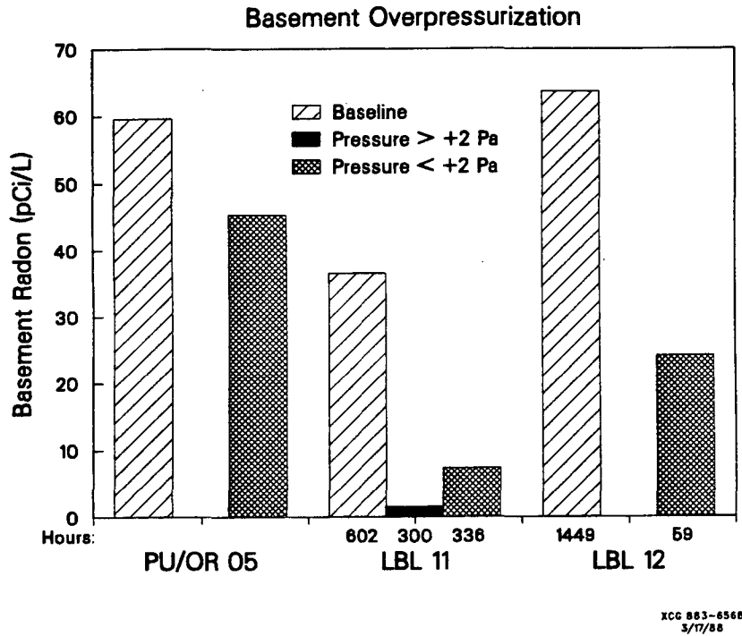
Figure 9. Reductions in basement radon levels due to basement overpressurization in three homes. Only when sufficient overpressures were achieved, did radon concentrations fall below target levels, as in the case of LBL11.
