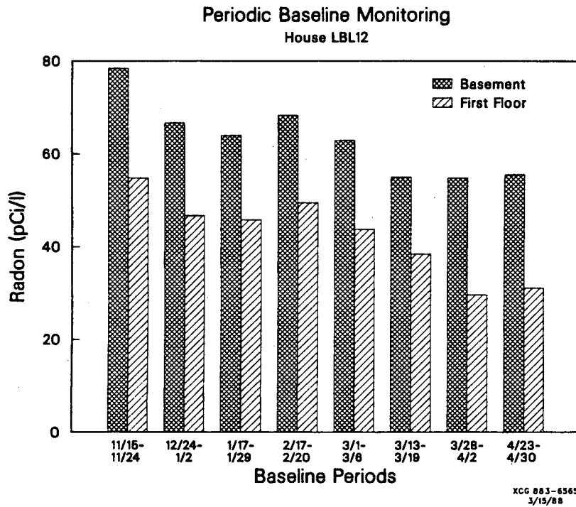
Figure 3. Baseline radon concentrations for LBL12. Falling radon levels throughout the heating season are typical, but not always the case, for the other homes.
