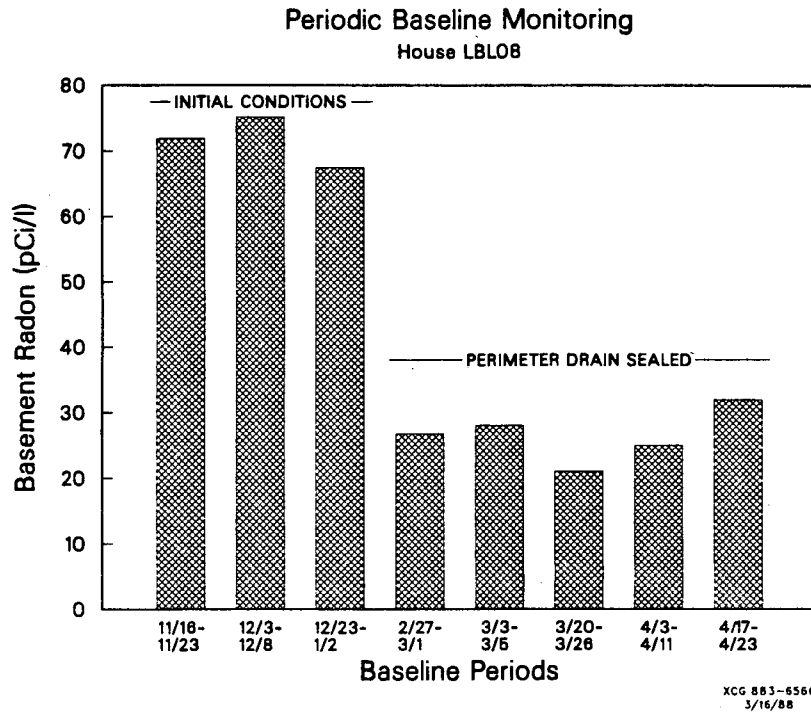
Figure 2. Baseline radon concentrations in the basement for LBL08. Note the decrease in the concentrations after the french drain was covered over. Each bar represents an average of approximately six days of continuous data.
