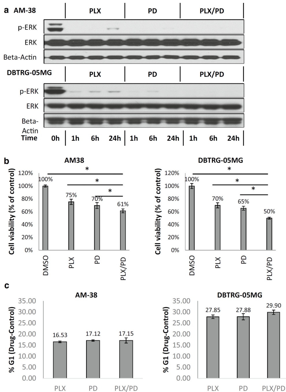
Fig. 2. Combined BRAF V600E and MEK inhibition prevented ERK recovery, decreased cell viability, and increased G1 phase arrest in BRAF V600E glioma cell lines. All treatments used DMSO (control), 2 \mu M PLX4720, 10 nM PD0325901 and their combination. a AM-38 and DBTRG-05MG cells were cultured in 10% serum media overnight, then treated for 0, 1, 6 and 24 h. Cell lysates were analyzed by western blot. In both AM-38 and DBTRG-05MG cell lines, combined treatment decreased the recovery of p-ERK induced by PLX4720. b AM-38 and DBTRG-05MG cells were treated for 5 days. Media was changed once every 3
