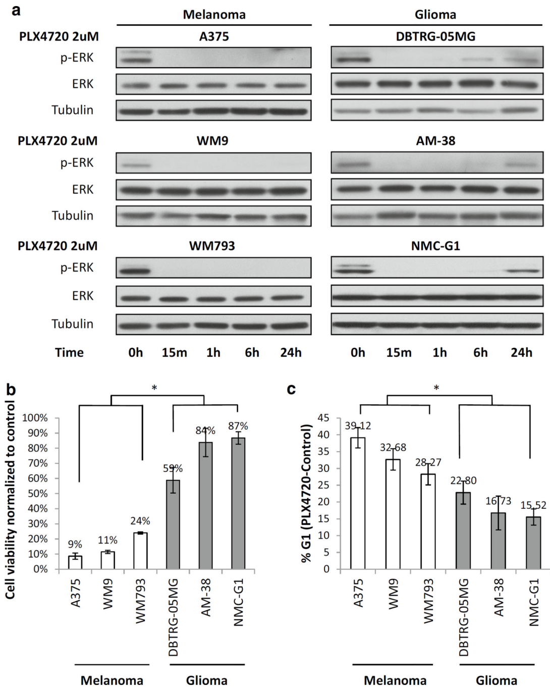
Fig. 1. Efficacy of PLX4720 against BRAF V600E melanoma and glioma cells. BRAF V600E -mutant glioma cells (DBTRG-05MG, AM-38 and NMC-G1) and BRAF V600E -mutant melanoma cells (A375, WM9 and WM793) were used. a Cells were cultured in 10% serum media, and treated with 2 \mu M PLX4720 for 0 h, 15 m, 1, 6, and 24 h. Cell lysates were analyzed using western blot. Phosphorylation of ERK was inhibited by PLX4720 initially in all cell lines, but partially recovered in glioma cell lines compared to in melanoma cell lines. b Cells were treated with DMSO (control) or 2 \mu M PLX4720 for 6 days. Media was changed once every
