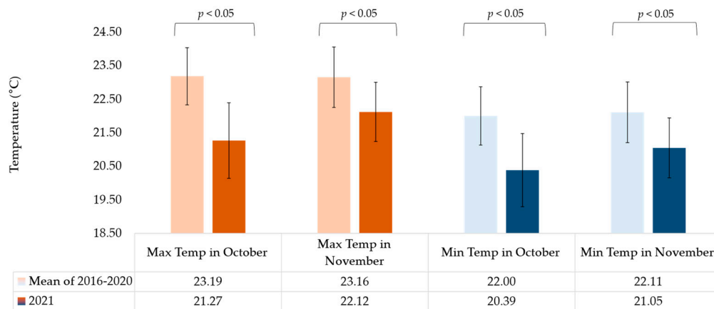
Figure 3. Maximum and minimum temperatures recorded across the State of Rio de Janeiro for October and November from 2016 to 2021. Data from 2016–2020 and 2021 were averaged between ten weather stations covering the State of Rio de Janeiro. The data for the mean of 2016–2020 represent all measurements taken from maximum and minimum temperatures for the ten weather stations in Rio de Janeiro. A Wilcoxon signed rank test was performed comparing 2021 maximum and minimum temperatures for the months of October and November with that of the mean of 2016–2020. Error bars represent standard error. All p -values were <0.001.
