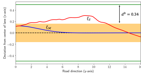
Figure 7.8. The green lines represent the boundaries of the original reach set. The yellow region is the contracted reach set for the model computed using \hat{d}_\epsilon . The model’s trajectory shown in blue is entirely contained within the yellow region. Consequently, the system’s trajectory (shown in dotted red) leaves the yellow region but is contained within the original reach set at all times.
