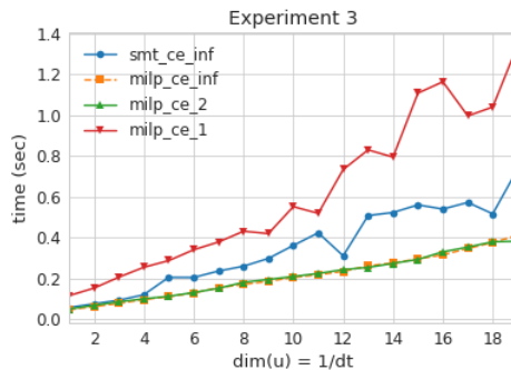
Figure 3.10. The x -axis shows the dimension of the input space, while the y -axis shows the time taken for the CEGIS loop to converge. milp\_ce\_1 refers to \mathcal{C}_H^{k=1} , milp\_ce\_2 refers to \mathcal{C}_H^{k=2} , milp\_ce\_inf refers to \mathcal{C}_N , and smt\_ce\_inf refers to \mathcal{C}_D .
