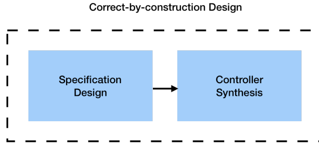
Figure 1.1. Correct-by-construction design
