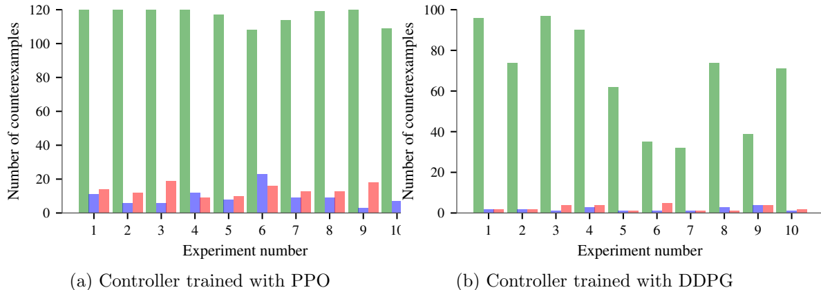
Figure 6.7. The green, blue and red bars show the number of counterexamples generated when modeling \rho_{\mu_1}, \rho_{\mu_2}, \rho_{\mu_3} as separate GPs, modeling \rho_{\varphi} as a GP and random testing respectively for the mountain car example (Sec 6.6.3.2). While our modeling paradigm, finds orders of magnitude more counterexample compared to the other two methods, we notice that modeling \rho_{\varphi} as a single GP performs much worse than random sampling for the controller trained with PPO Fig 6.7a and comparable for the controller trained with DDPG Fig 6.7b.
