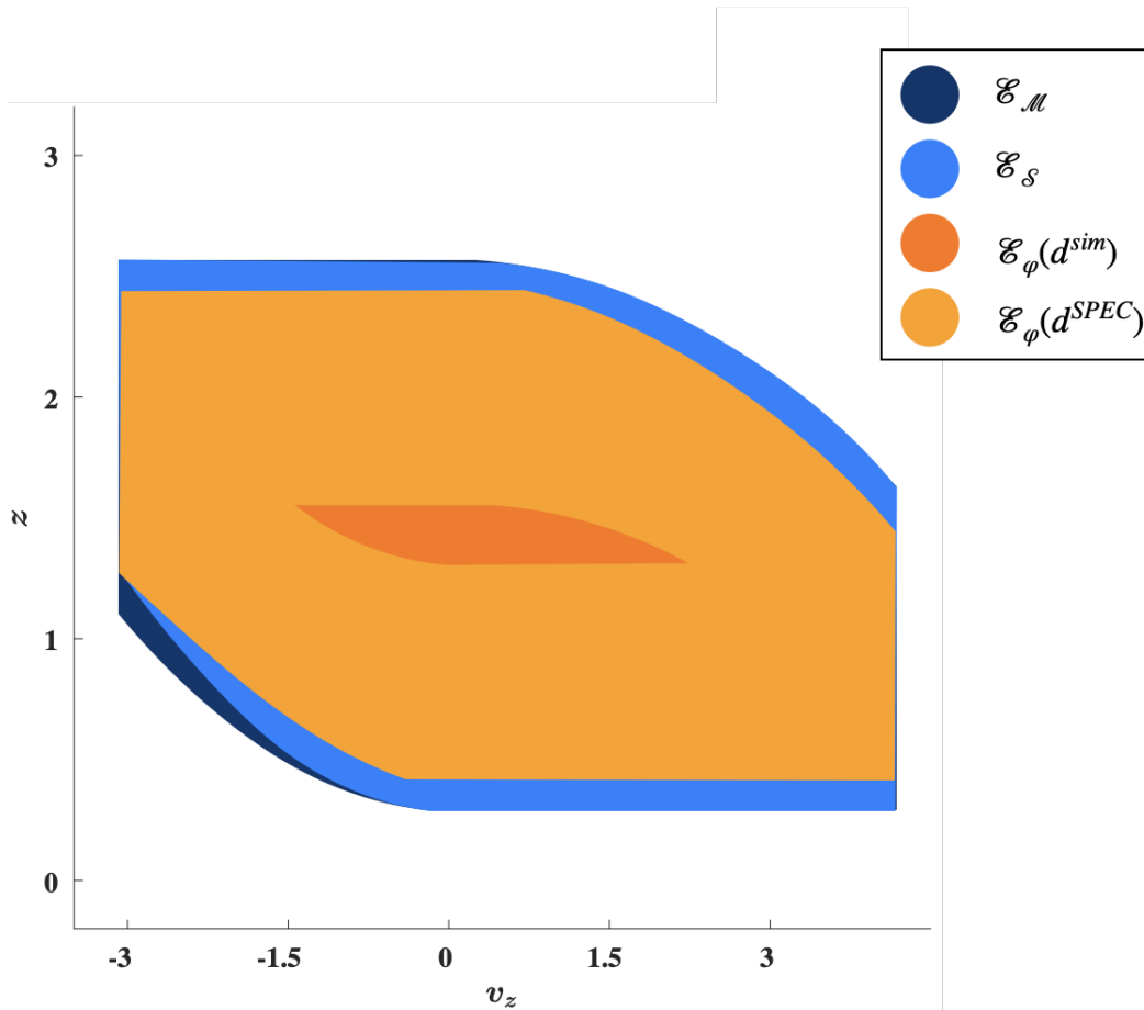
Figure 7.5. Different reachable sets when the quadrotor abstraction is overly optimistic. Here we compute the exact reach sets corresponding to \mathcal{E}_{\mathcal{M}} , \mathcal{E}_{\mathcal{S}} , \mathcal{E}_{\varphi}(d^{SPEC}) and \mathcal{E}_{\varphi}(d^{sim}) . The distance metric d^{SPEC} achieves a far less conservative under-approximation of \mathcal{E}_{\mathcal{S}} compared to d^{sim} .
