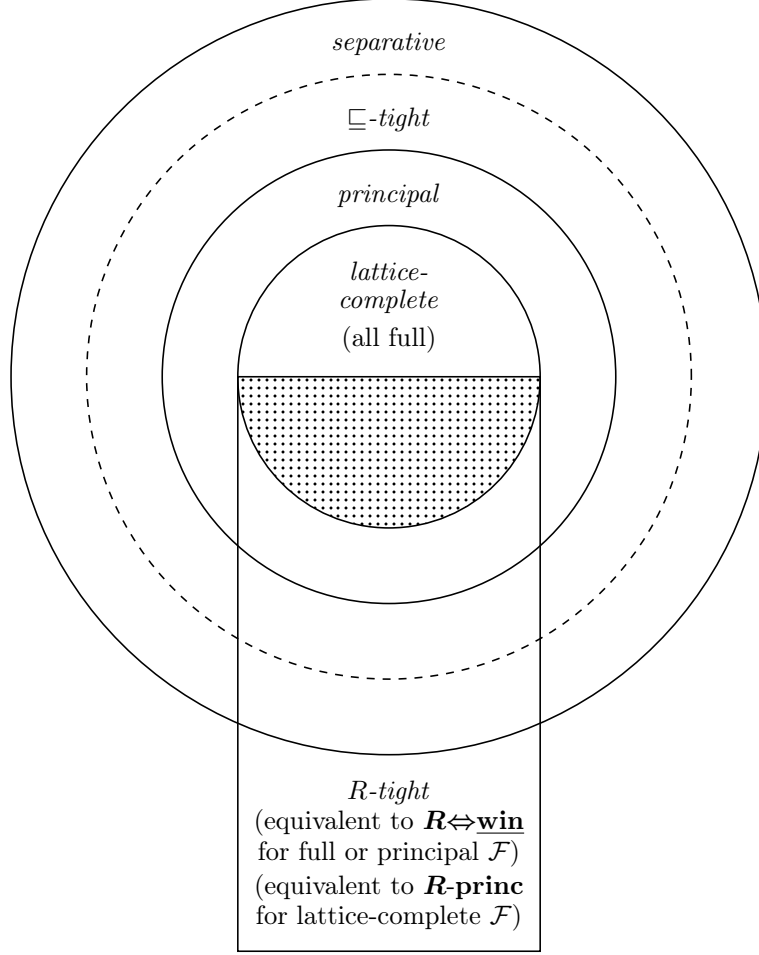
Figure 4.1: rich frames (dotted region) shown inside other frame classes from § 4. Each label applies to everything inside the smallest circle (or rectangle) that contains the label. The dashed circle reflects the fact that the distinction between separative and \square - tight disappears for full possibility frames (Fact 4.33).
