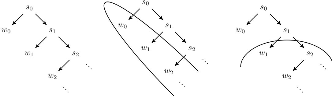
Figure 2.4: the Beth comb (left) and two examples of non-regular-open sets (middle and right).
