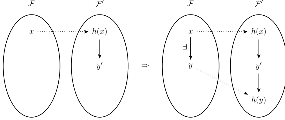
Figure 3.1: the \square -back condition of strict possibility morphisms. Dotted lines indicate the possibility morphism h , while a solid line from s down to t indicates that t is a refinement of s .
