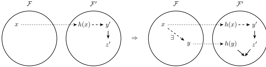
Figure 3.1: the \square -back condition of strict possibility morphisms. Dotted lines indicate the possibility morphism h , while a solid line from s down to t indicates that t is a refinement of s .
