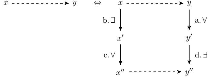
Figure 2.10: \mathbf{R} \Leftrightarrow \mathbf{win}
