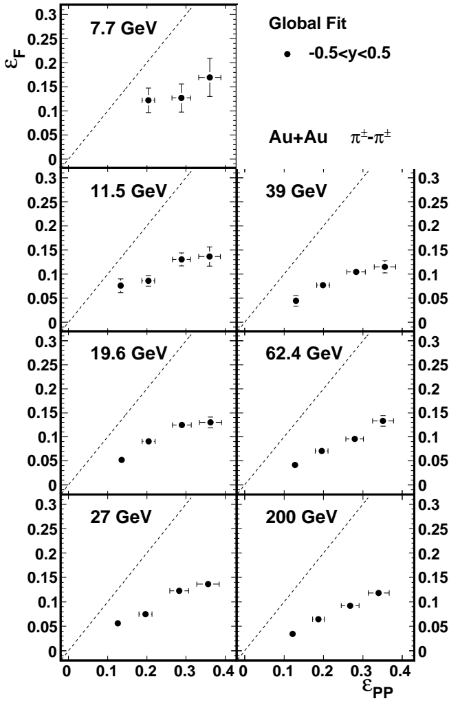
FIG. 26: The eccentricity of the collisions at kinetic freeze-out, \varepsilon_F , as a function of initial eccentricity relative to the participant plane, \varepsilon_{PP} , at mid-rapidity. All results are for \langle k_T \rangle \approx 0.31 GeV/c. Error bars include only statistical uncertainties. The line has a slope of one indicating no change in shape. Points further below the line evolve more to a round shape.
