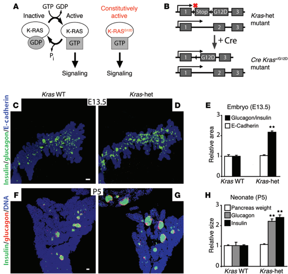
Figure 1. Pancreatic endocrine mass in Kras-het mice. (A and B) Schematic in A illustrates the relationship between K-RAS-GTP binding and intracellular signaling; schematic in B illustrates the conversion of the transcriptionally silent Kras G12D -knock-in allele, which contains the G12D mutation in exon 2 and an upstream LoxP-Stop-LoxP sequence (12), to an active allele expressing constitutively active K-RAS G12D after Cre-mediated recombination. (C and D) Projection images of the dorsal pancreas were collected by whole-mount confocal microscopy from E13.5 mouse embryos of the indicated genotypes and immunostained for E-cadherin (blue) and glucagon and insulin (green) ( n = 6 Kras WT, n = 6 Kras-het ). (E) Quantification of immunostained areas in the epithelial pancreas (E-cadherin) and endocrine pancreas (glucagon and insulin) relative to WT embryos. (F–H) Pancreatic sections from P5 WT (F) and Kras-het (G) neonates were immunostained for glucagon (red) and insulin (green), with quantification of the relative insulin and glucagon areas and pancreatic mass (H) ( n = 3 Kras WT, n = 3 Kras-het ). All data points represent the mean ± SEM. ** P < 0.01 versus WT animals by 2-tailed Student’s t test. Scale bars: 50 μm.
