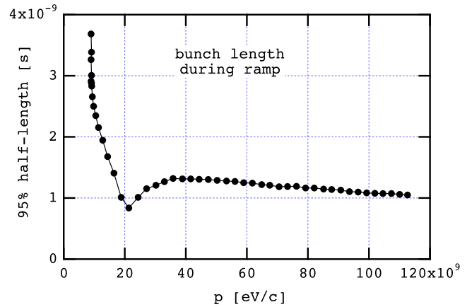
Figure 2: Bunch length vs. beam momentum during the MI ramp. Transition is crossed just above 20 GeV/c.
