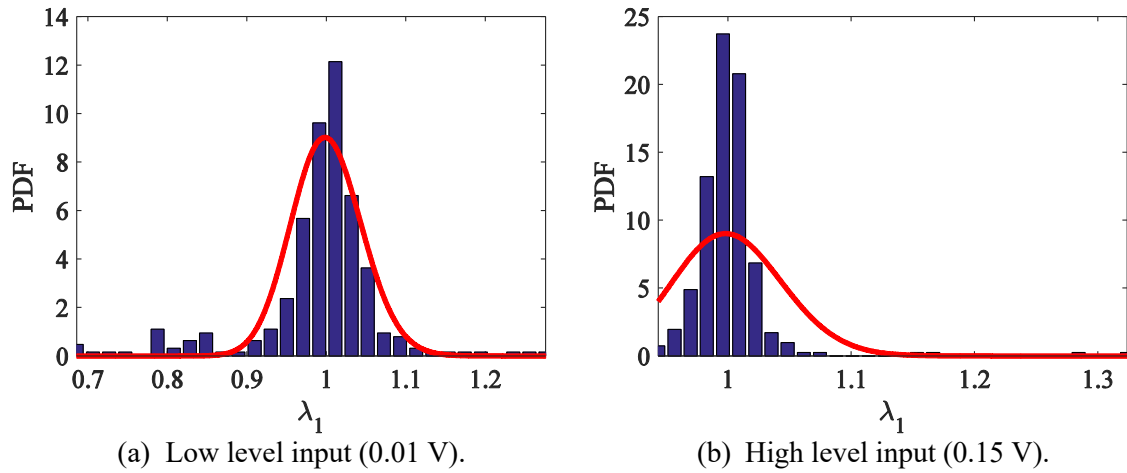
Figure 15. Distribution of the experimental linear damage index compared to the theoretical distribution for the reference case. The blue bar represents the experimental data and the continuous line — represents the theoretical distribution.
