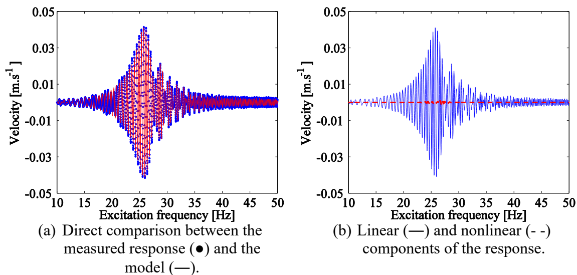
Figure 9. Response of the Volterra model to a low level excitation (0.01 V).
