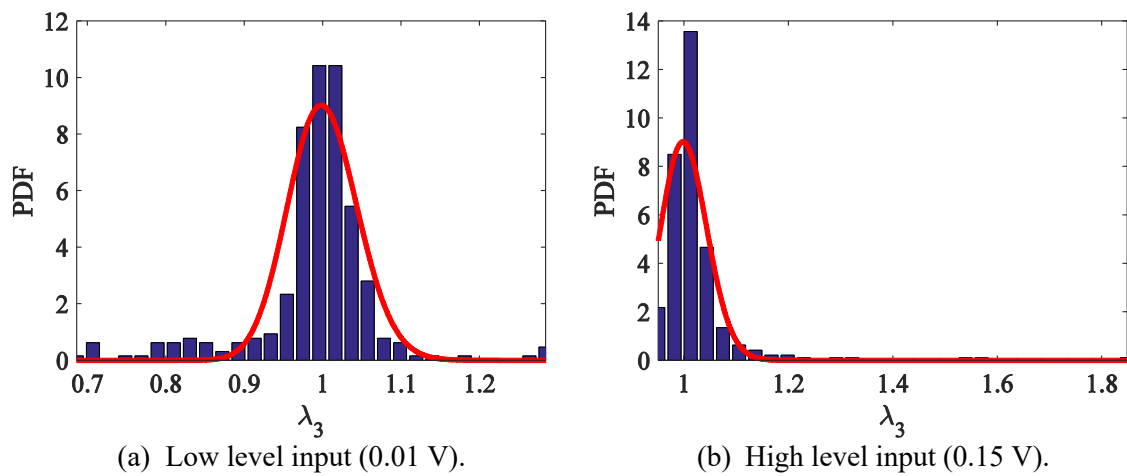
Figure 16. Distribution of the experimental nonlinear damage index compared to the theoretical distribution for the reference case. The blue bar represents the experimental data and the continuous line — represents the theoretical distribution.
