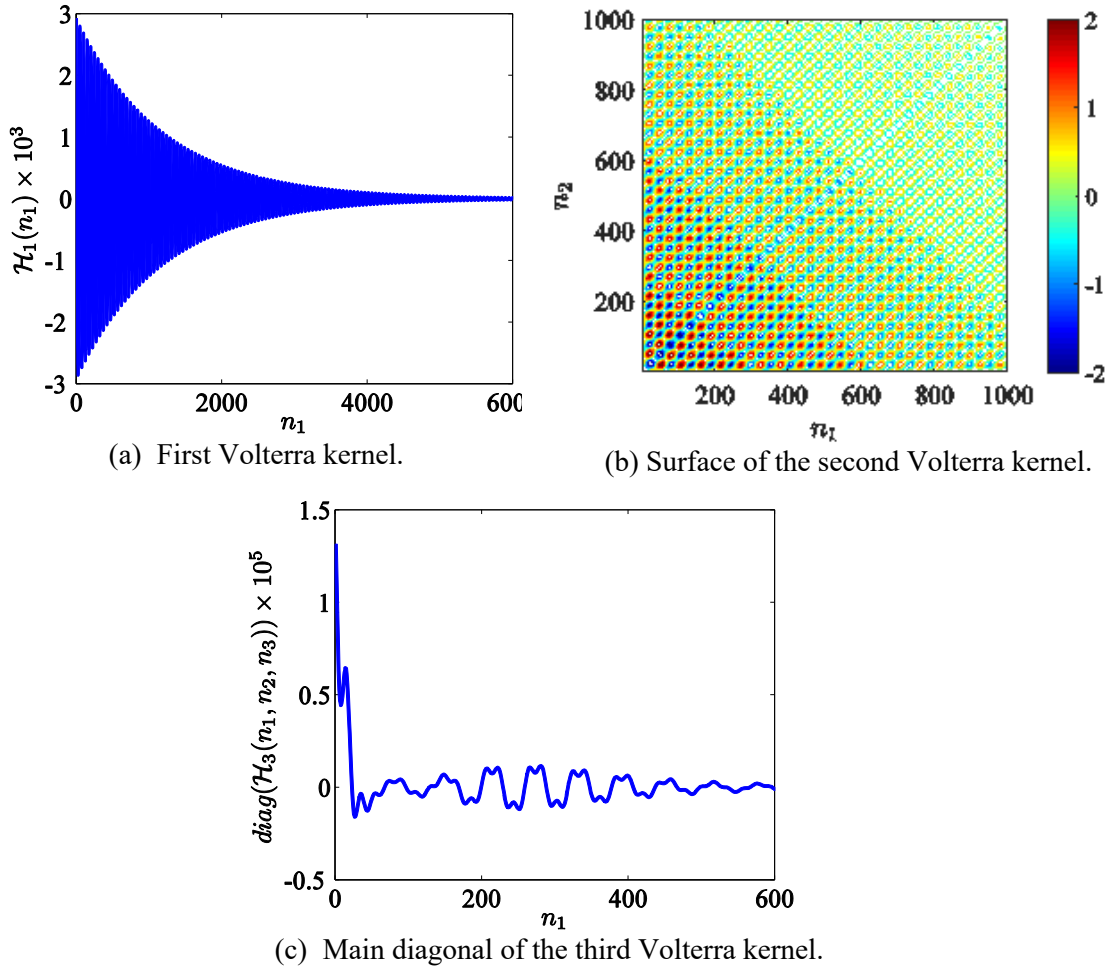
Figure 8. Representation of the Volterra kernels in the physical basis.
