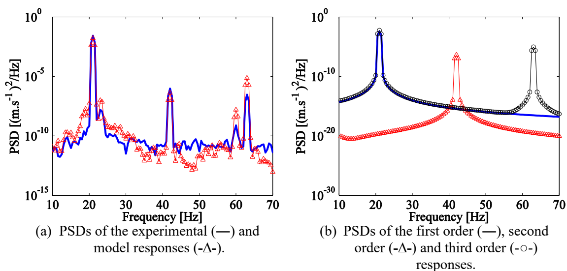
Figure 11. PSD of the response of the Volterra model to a sine excitation in the linear natural frequency of the structure.
