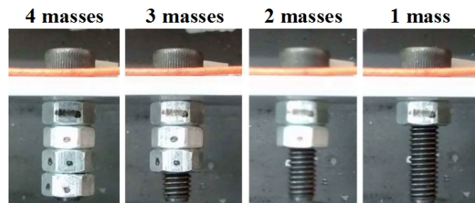
Figure 12. Illustration of the damage simulation.
