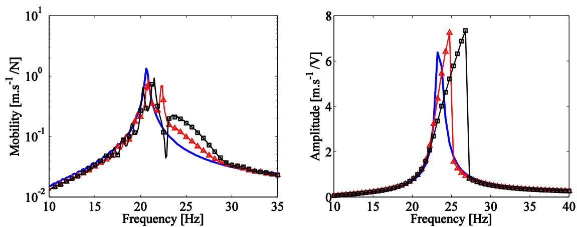
(a) FRF of the system excited with a chirp excitation.
