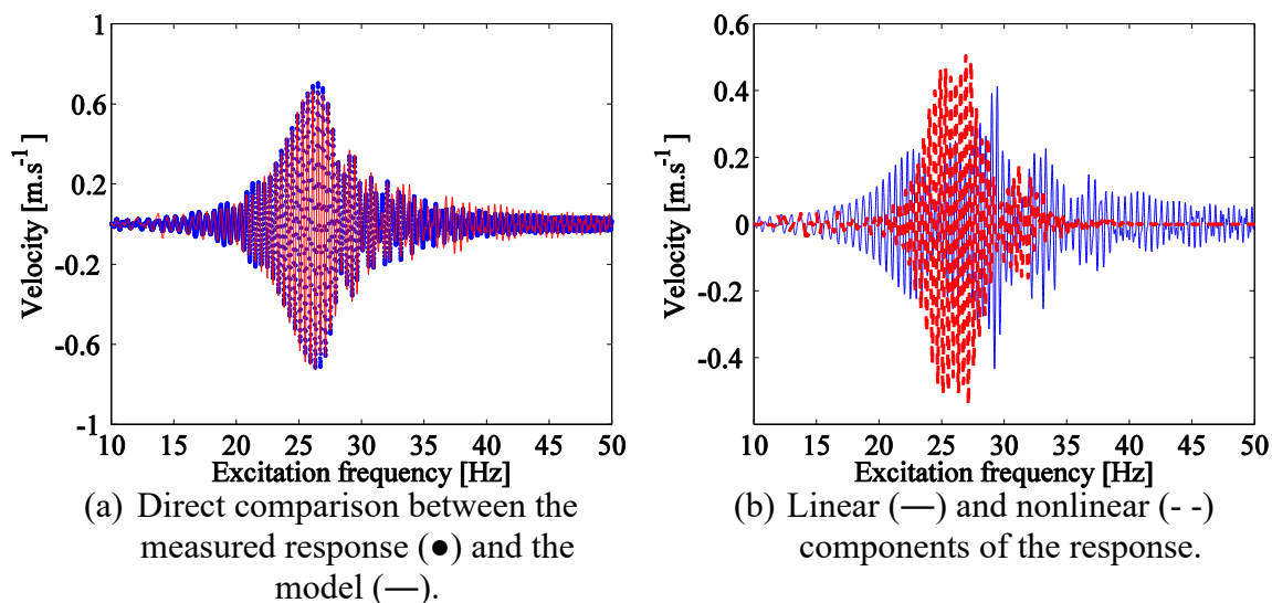
Figure 10. Response of the Volterra model to a high level excitation (0.15 V).
