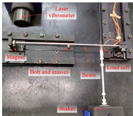
Figure 2. Picture of the experimental setup.
