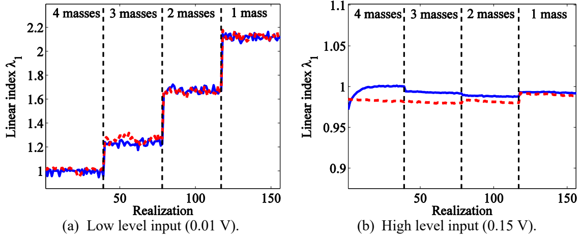
Figure 13. Linear index under two different input levels. The continuous line — is representing the indexes during the damage application (states 1 to 4) and - - represents the indexes during the repair (states 5 to 8).
