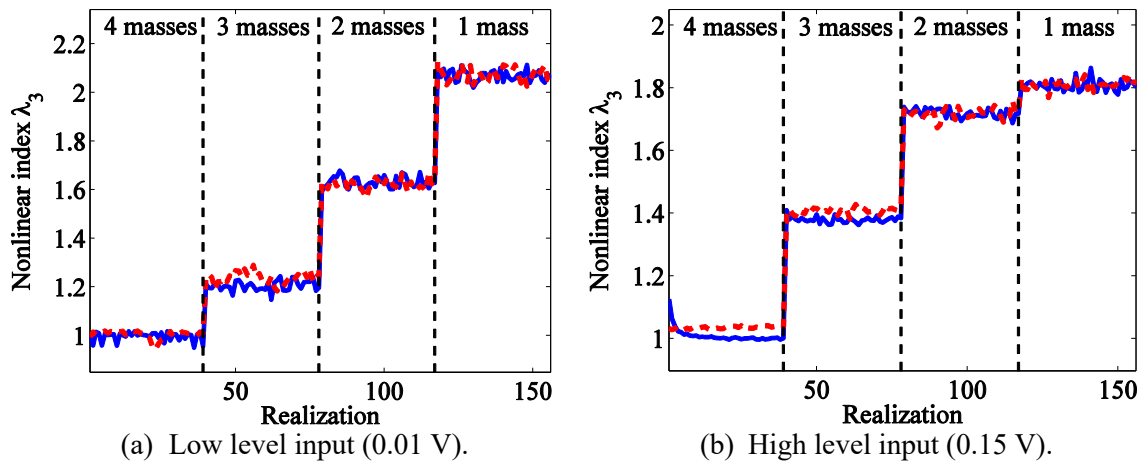
Figure 14. Nonlinear index under two different input levels. The continuous line — is representing the indexes during the damage application (states 1 to 4) and - - represents the indexes during the repair (states 5 to 8).
