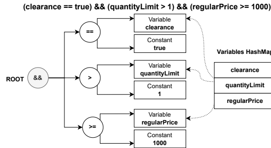
Figure 3.5: Example filter expression tree and variables map
