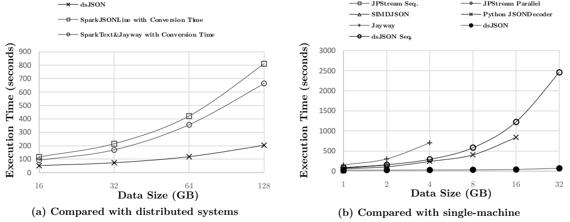
Figure 3.8: Processing time with increasing input size
