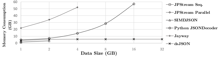
Figure 3.9: Memory usage compared to single machine parsers
