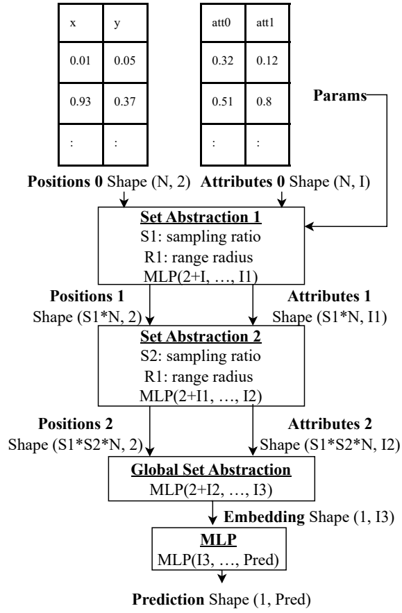
Figure 4.2: GeoGraph architecture
