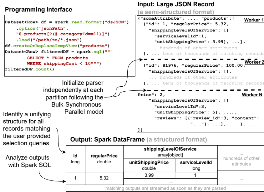
Figure 3.1: An example highlighting dsJSON processing steps
