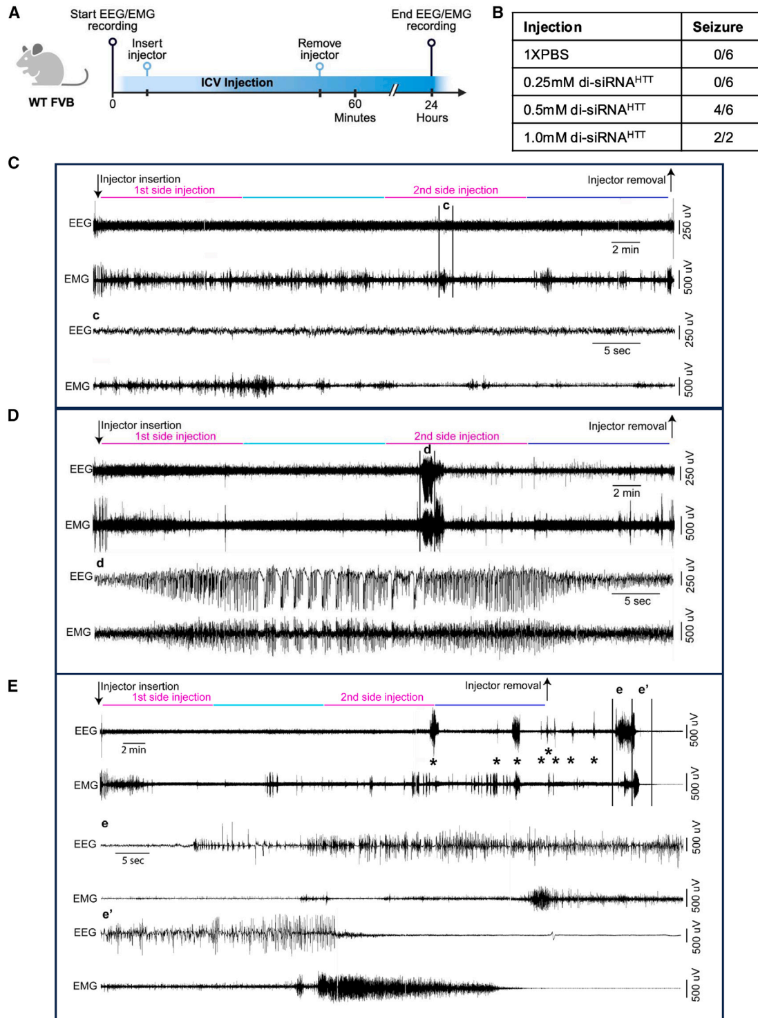
Figure 2. Electrophysiology defines the acute neurotoxicity induced by CNS injections of di-siRNA in awake mice
