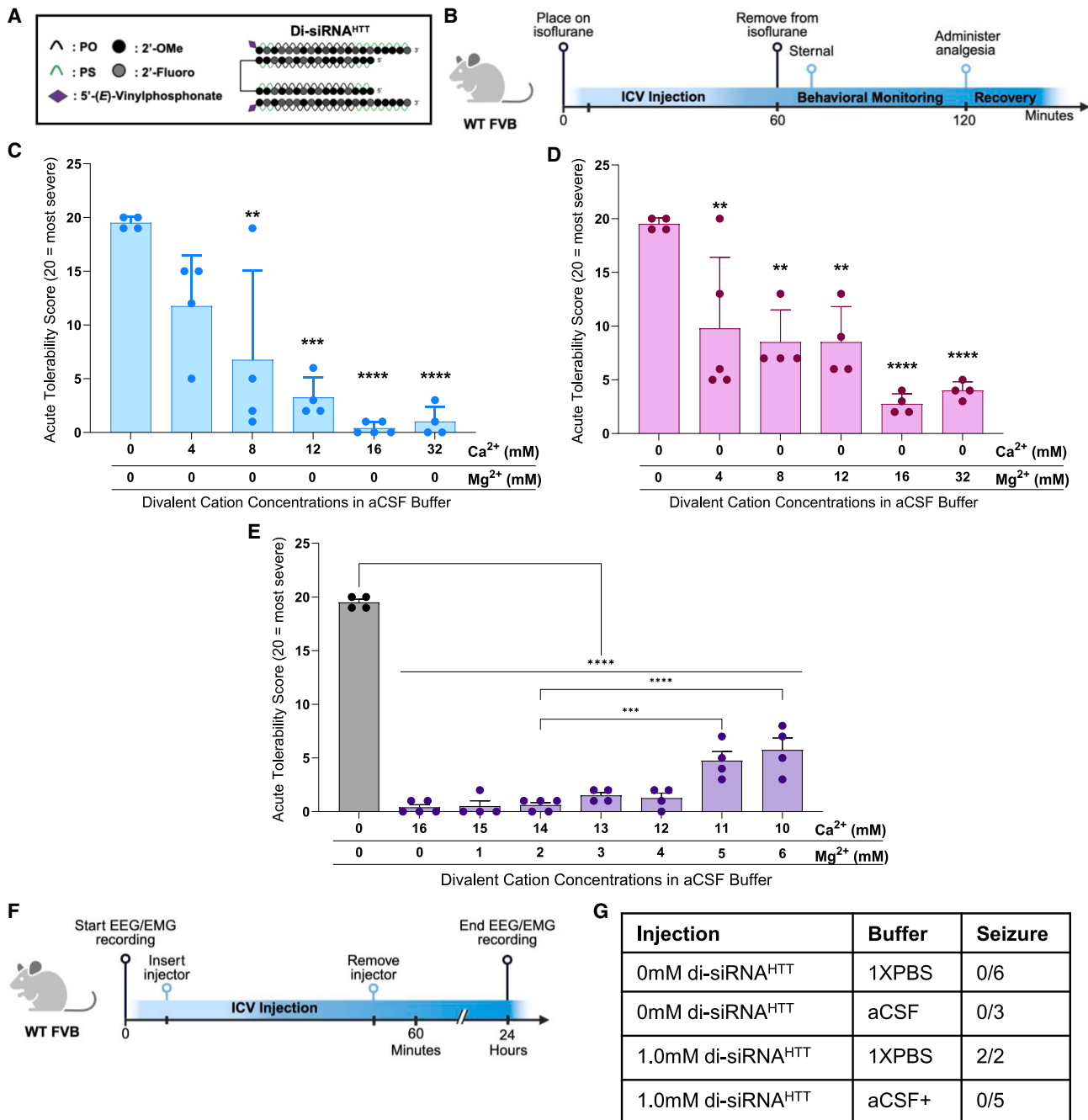
Figure 4. The acute neurotoxicity is preventable by adding Ca 2+ and Mg 2+ to aCSF buffer
