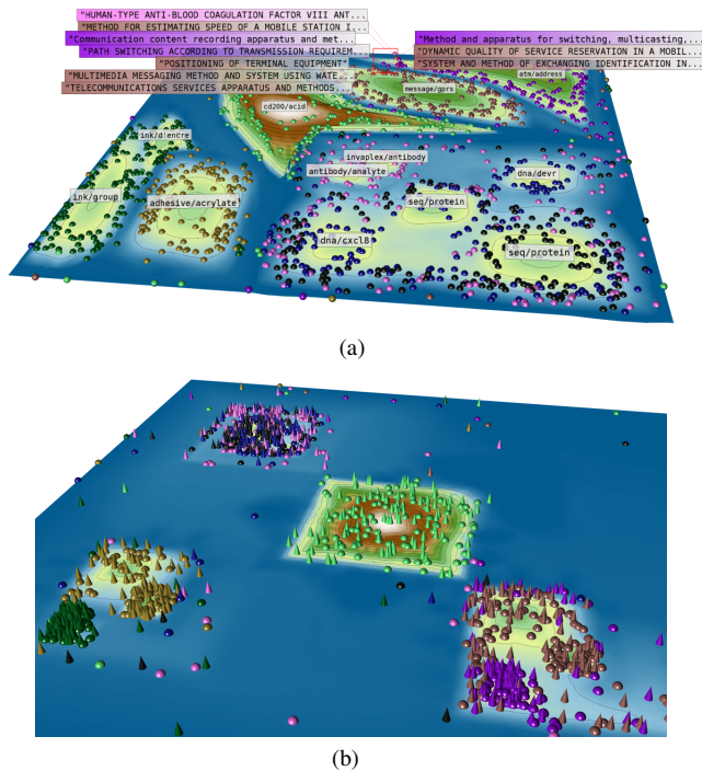
Figure 6: (a) 2-D topological landscape of the patent data set. The nesting structure of the islands reflects the IPC hierarchy of the test data set. (b) The same landscape without volumetric distortion. Even by learning the LDA with only 50% of the input data, the remaining patents (the cones) are placed on their correct islands (clusters).
