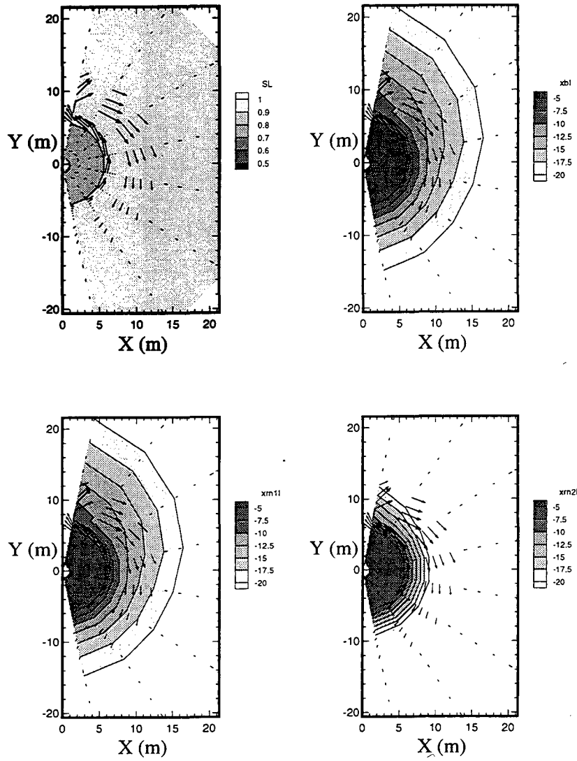
Fig. 5. Liquid saturation, and log mass fraction brine, parent (rn1), and daughter (rn2) in the liquid phase after 1 yr. Vectors show the aqueous phase velocity.
