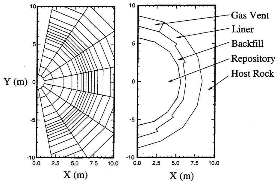
Fig. 2. Closeup of repository region showing spider mesh connections (left), and the domain boundaries for the gas vent, liner, backfill, repository, and a small portion of host rock (right).
