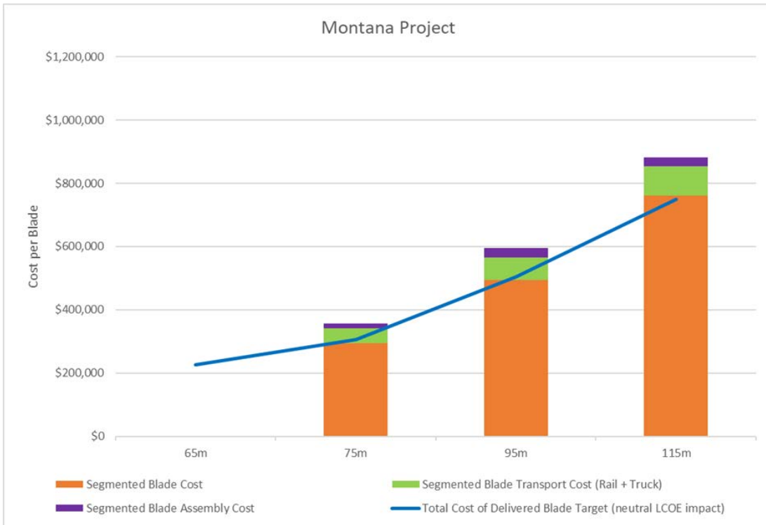
Figure 8-11 Total cost of delivered segmented blades - Montana
