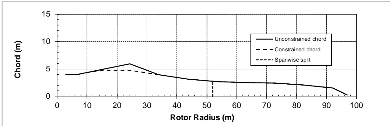
Figure 6-2 Spanwise and chordwise joint locations for 95 m blade
