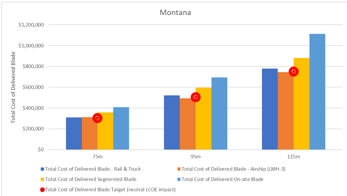
Figure 9-2 Innovation Pathway summary – Total cost of delivered blades, Montana
