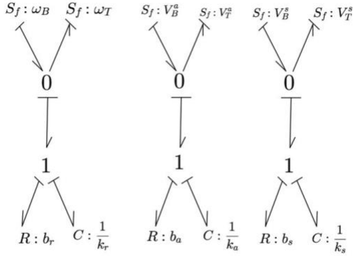
Figure 8. Complementary Bond Graph connecting two consecutive inertias
