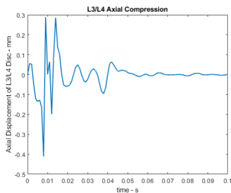
Figure 10. L3/L4 segment's axial compression
