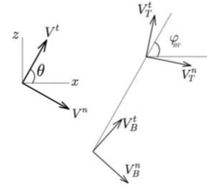
Figure 5. geometric diagram of two consecutive inertias T (top) and B (bottom), and their body-fixed coordinates
