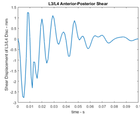
Figure 11. L3/L4 segment's shear displacement
