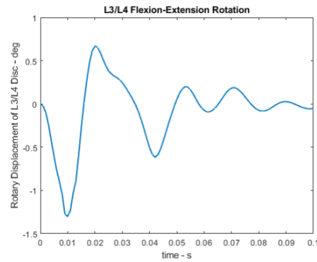
Figure 12. L3/L4 segment's rotary displacement
