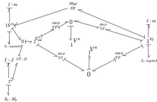
Figure 7. Bond Graph for a typical vertebra
