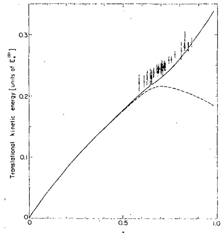
Fig. 2. Calculated and experimental fission-fragment kinetic energies.
