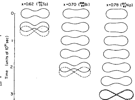
Fig. 1. Illustrations of the descent from saddle to scission.
