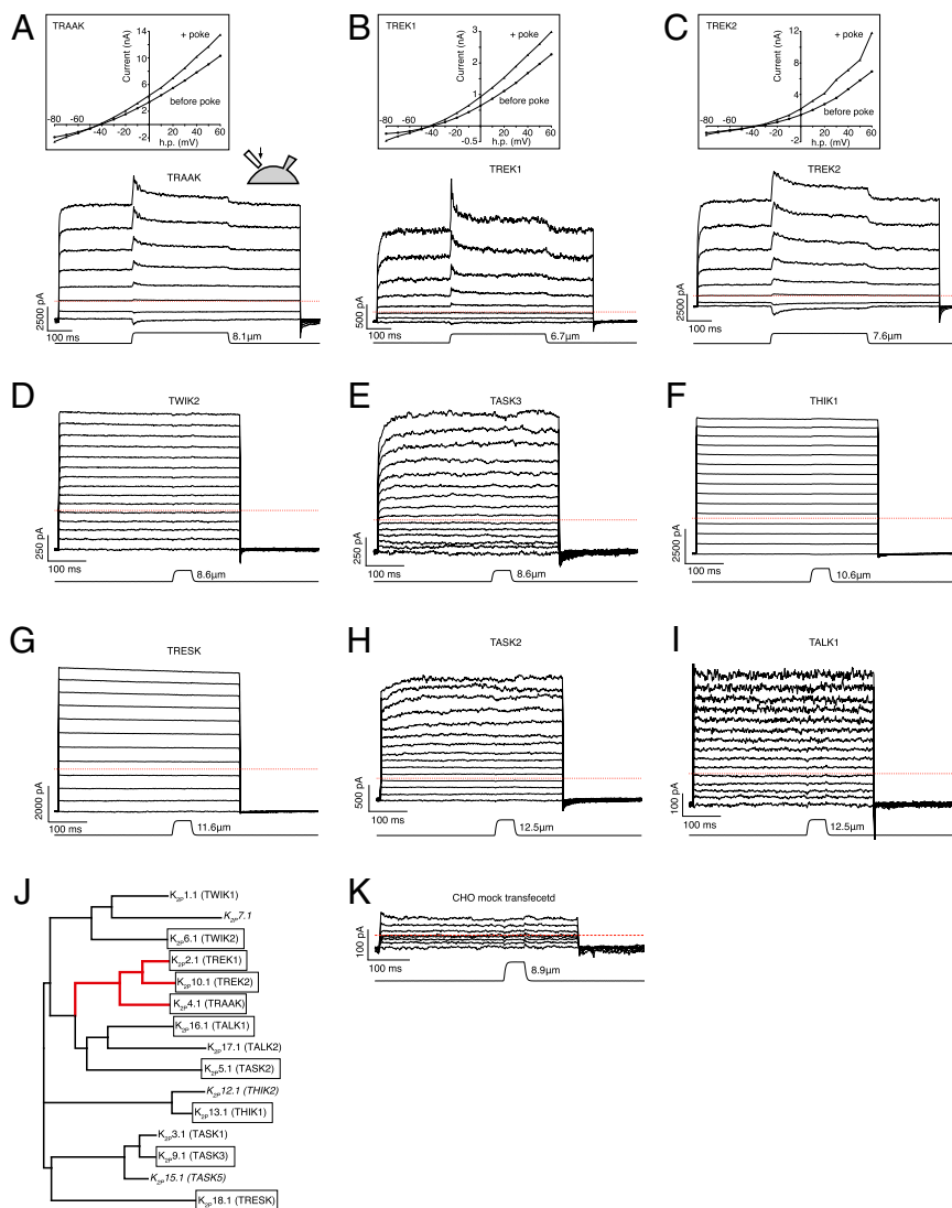
Fig. 2. Only TRAAK and TREK K2Ps are activated by mechanical force applied to cells. ( A–I and K ) Whole-cell current response ( Upper ) to mechanical stimulation recorded from a cell expressing (A) TRAAK, (B) TREK1, (C) TREK2, (D) TWIK2, (E) TASK3, (F) THIK1, (G) TRESK, (H) TASK2, (I) TALK1, or (K) a mock-transfected CHO cell during a voltage step protocol ( V_h = -80 mV, -80 to +60 mV, \Delta V = 10 mV) during which a glass probe was depressed against the cellular membrane ( Lower ). Successive voltage steps were separated by 5 s. Traces every 20 mV are shown in A–C and every 10 mV in D–I . ( A–C , Insets ) Mean current before mechanical stimulation and peak current during mechanical stimulation recorded at each holding voltage are plotted from experiments shown in A–C . ( J ) Phylogenetic tree of the 15 human K2Ps (adapted from ref. 25). The TRAAK–TREK clade is highlighted red. Channels for which data are presented in A–I are boxed. Channels for which functional expression has not been reported are italicized. Experiments in A–I and K were performed with internal 150 mM K^+ , 0 mM Na^+ and external 135 mM Na^+ , 15 mM K^+ . All recordings are representative of at least three separate experiments.
