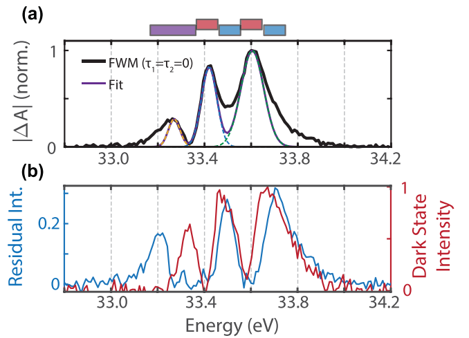
FIG. 6. Deconvolution of core-exciton four-wave mixing (FWM) signals. Spectral deconvolution of the time-zero spectrum with core-excitonic components identified in both the bright and dark state scans. (a) Temporal overlap FWM spectrum (black) fit with the three primary core-excitons identified in the bright state scans with Gaussian distributions and (b) the fit residuals (blue, left axis) compared with the core-excitons (normalized, red, right axis) identified in the dark state scans following overlap at a 7 fs delay. The blocks above the top plot highlight the five distinct core-excitonic regions discussed in the text. The red blocks refer to distinct states observed only in the bright state scan in (a); blue blocks refer to distinct states identified through the comparison of the residuals and dark state scans in (b) and the purple block on the low energy region highlights features observed in both (a) and (b), which may correspond to more than one distinct state.
