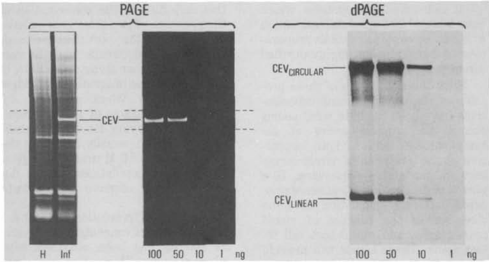
Fig. 1. Polyacrylamide gel electrophoresis under standard (PAGE) and denaturing conditions (dPAGE) in the presence of 8M urea. Gels containing nucleic acid preparations (2M LiCl soluble) from healthy (H) and CEV infected (Inf) tissues (left) or a standard concentration series of purified CEV (middle) were stained with ethidium bromide after electrophoresis to determine position of CEV. For analysis by sequential electrophoresis on dPAGE, gel segment containing CEV band was excised as indicated (---) and applied to the top of a second gel for dPAGE. Resolution of the circular and linear forms of CEV as well as the increased sensitivity of silver staining is presented in the gel at the right.
