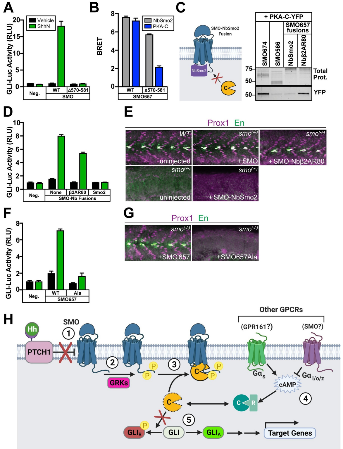
Fig 7. Hh signal transduction is blocked when SMO cannot bind PKA-C. (A) GLI transcriptional reporter assay in Smo -/- MEFs expressing wild-type SMO or SMOΔ570–581, treated with conditioned medium containing the N-terminal signaling domain of Sonic hedgehog (ShhN, green) or control, non-ShhN-containing conditioned medium (Vehicle, black). GFP serves as a negative control (“Neg.”). (B) BRET in HEK293 cells between nanoluc-tagged wild-type or Δ570–581 forms of SMO657 as donor, with YFP-tagged NbSmo2 (gray) or PKA-C (blue) as acceptor. (C) Left: Schematic of SMO-NbSmo2 fusion, predicted to block interactions with SMO that
