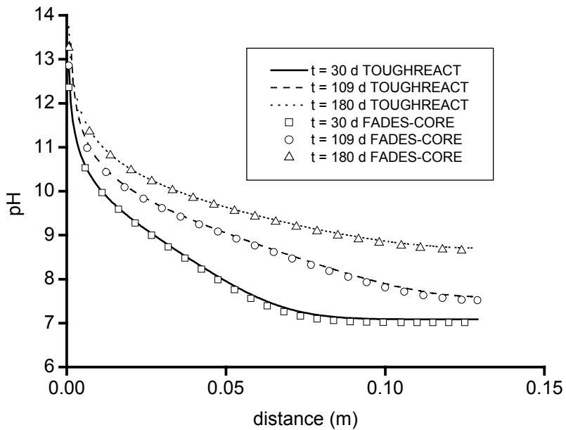
Figure 6. Comparison of pH distributions at different times obtained with TOUGHREACT and FADES-CORE for calcite dissolution case.
