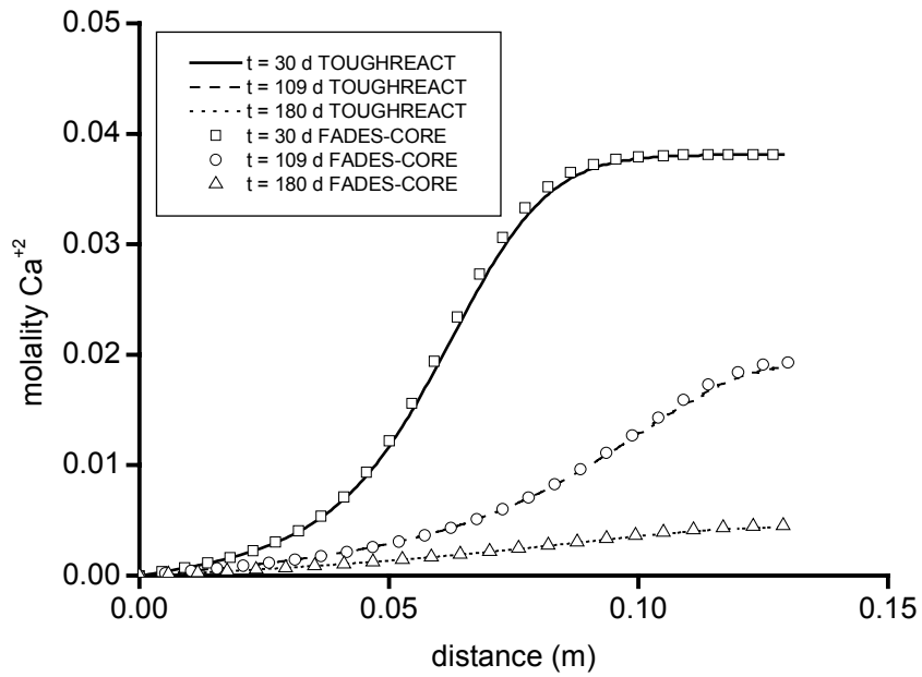
Figure 5. Comparison of \text{Ca}^{+2} concentration distributions at different times obtained with TOUGHREACT and FADES-CORE for calcite dissolution case.
