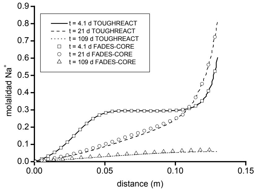
Figure 21. Comparison of \text{Na}^+ aqueous concentration distributions at different times obtained with TOUGHREACT and FADES-CORE.
