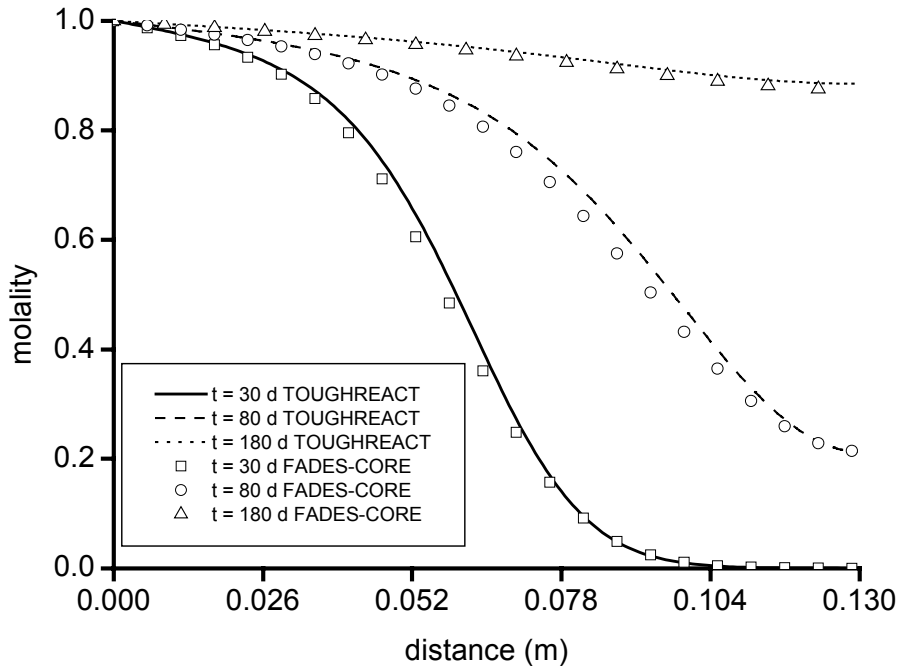
Figure 4. Comparison of concentration distributions at different times obtained with TOUGHREACT and FADES-CORE.
