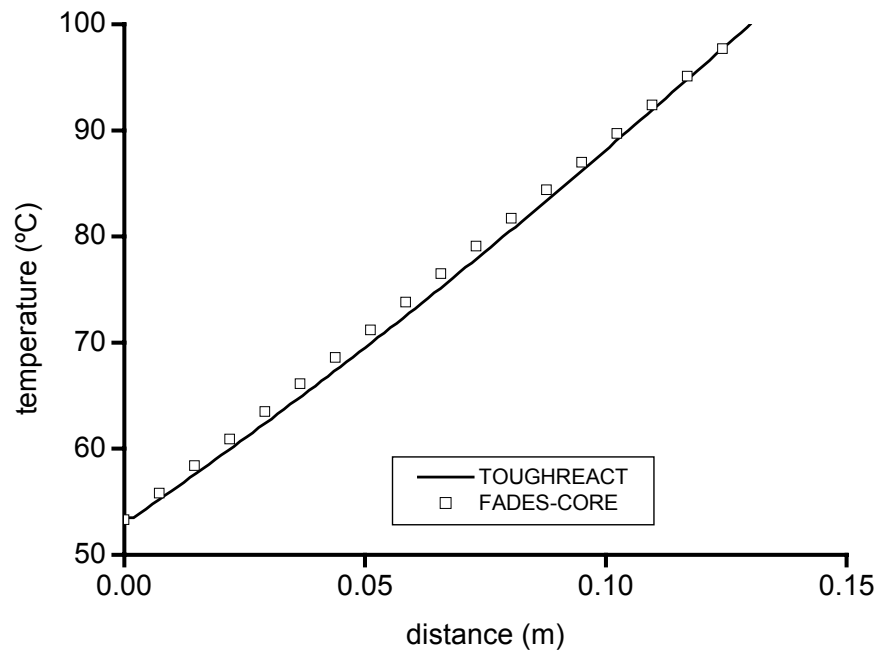
Figure 17. Comparison of temperature distributions obtained with TOUGHREACT and FADES-CORE with a steady-state heat transport.
