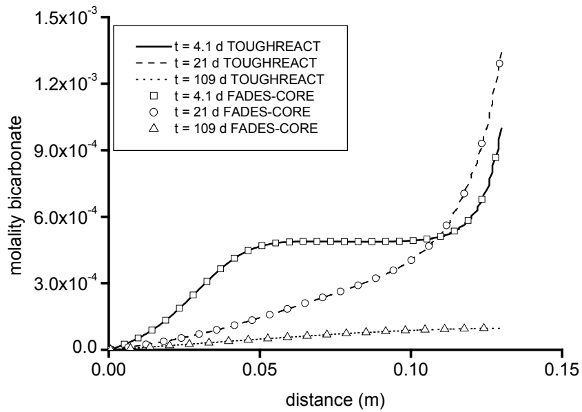
Figure 20. Comparison of bicarbonate aqueous concentration distributions obtained with TOUGHREACT and FADES-CORE at different times.
