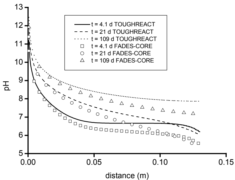
Figure 15. Comparison of pH concentration distribution at different times obtained with TOUGHREACT and FADES-CORE.
