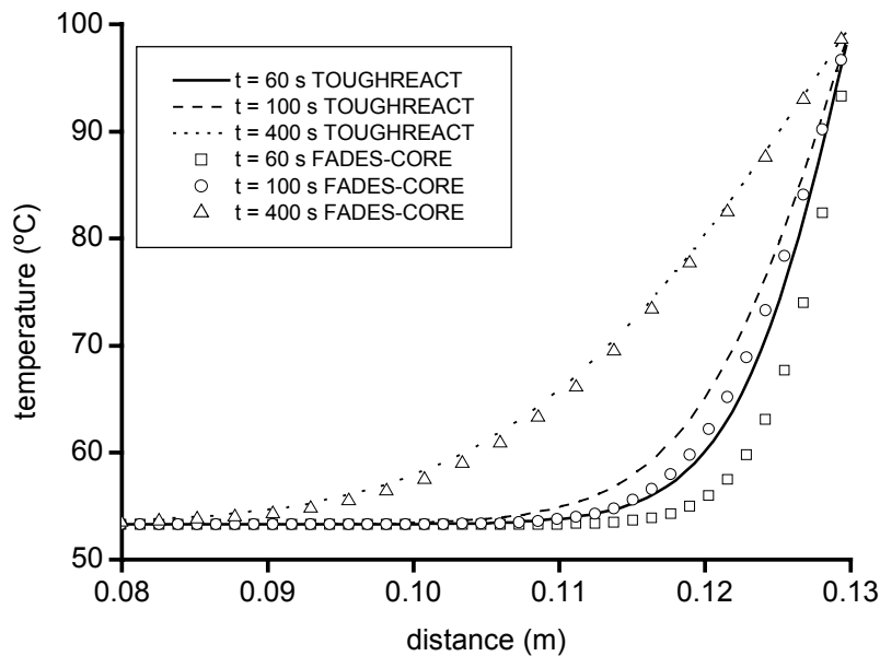
Figure 16. Comparison of temperature distributions at different times obtained with TOUGHREACT and FADES-CORE.
