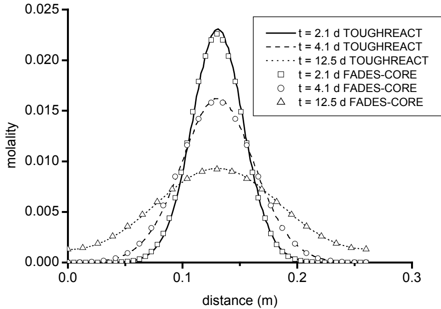
Figure 3. Comparison of concentration distributions at different times obtained with TOUGHREACT and FADES-CORE for the solute diffusion case.
