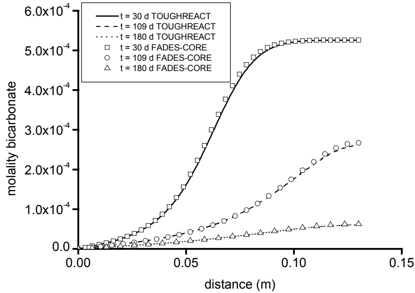
Figure 7. Comparison of bicarbonate concentration distributions at different times obtained with TOUGHREACT and FADES-CORE for calcite dissolution case.
