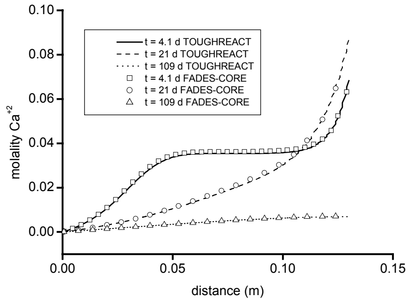
Figure 13. Comparison of \text{Ca}^{+2} concentration at different times obtained with TOUGHREACT and FADES-CORE.
