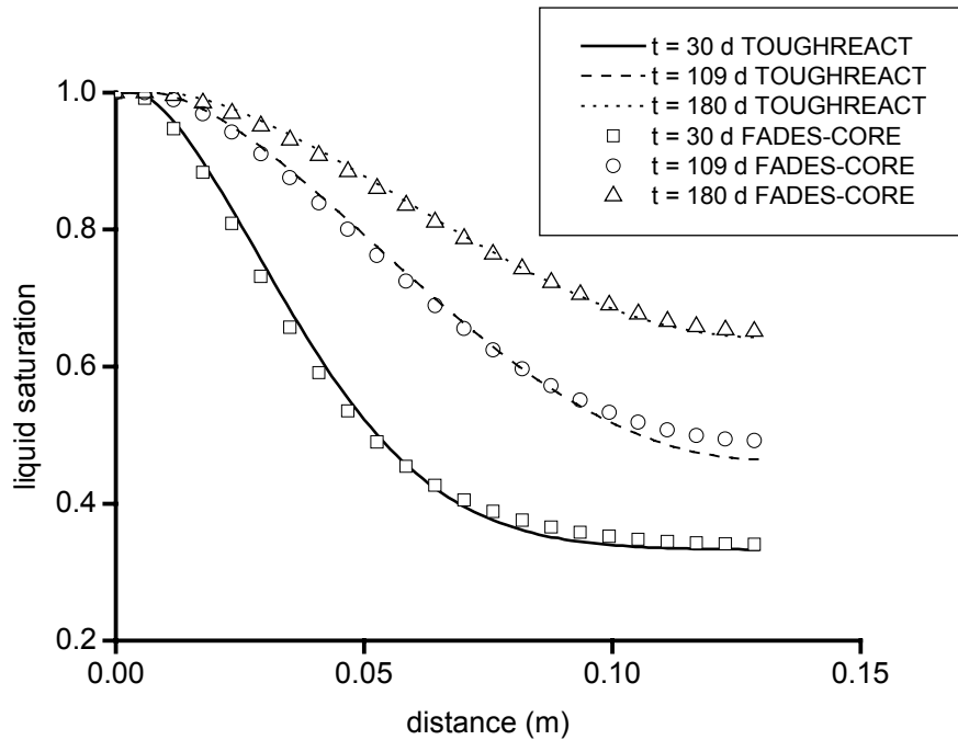
Figure 1. Spatial distribution of liquid saturation at different times obtained with TOUGHREACT and FADES-CORE.
