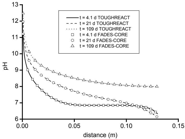
Figure 19. Comparison of pH concentration distributions at different times obtained with TOUGHREACT and FADES-CORE.
