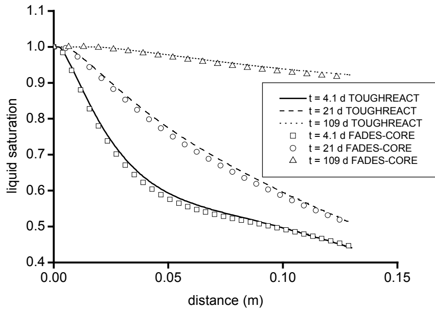
Figure 12. Comparison of liquid saturation obtained at different times with TOUGHREACT and FADES-CORE.
