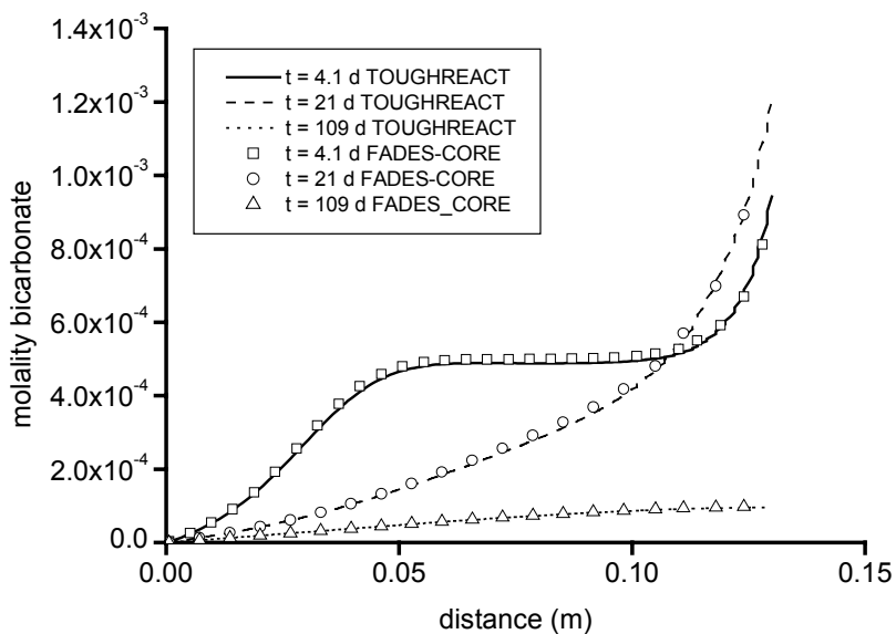
Figure 14. Comparison of bicarbonate concentration at different times obtained with TOUGHREACT and FADES-CORE.
