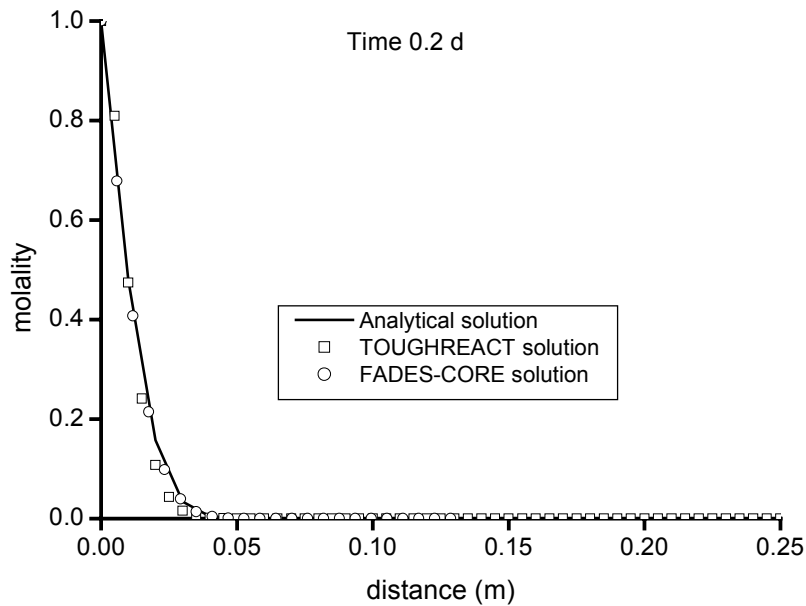
Figure 2. Comparison of analytical solution and concentration at 0.2 days obtained with TOUGHREACT and FADES-CORE.
