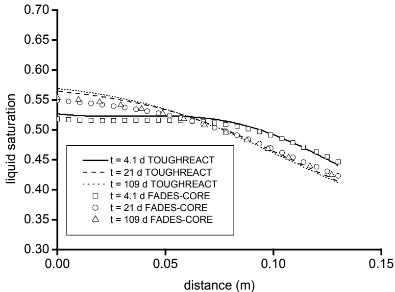
Figure 10. Comparison of liquid saturation distribution at different times obtained with TOUGHREACT and FADES-CORE.
