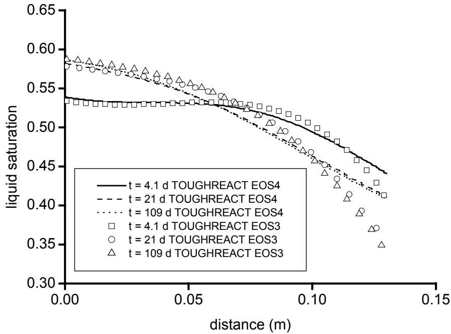
Figure 8. Comparison of liquid saturation distributions at different times using EOS3 and EOS4 modules with TOUGHREACT.
