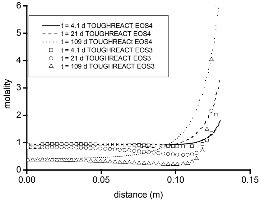
Figure 9. Comparison of molality distributions at different times using EOS3 and EOS4 modules with TOUGHREACT.
