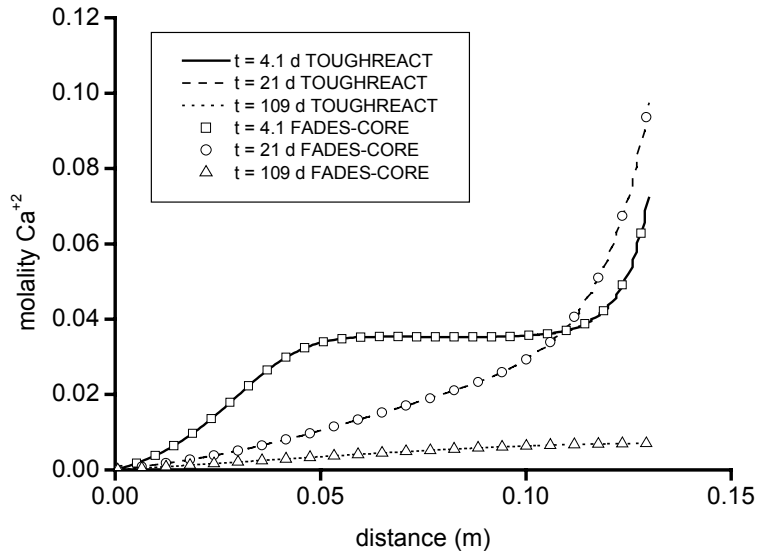
Figure 18. Comparison of \text{Ca}^{+2} aqueous concentration distributions at different times obtained with TOUGHREACT and FADES-CORE with a steady-state heat transport.
