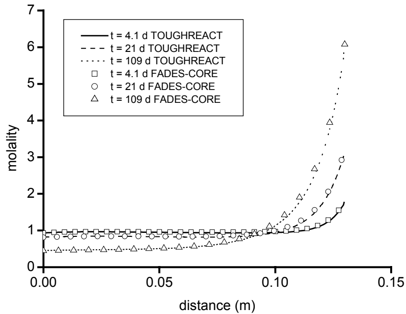
Figure 11. Comparison of molality distributions at different times obtained with TOUGHREACT and FADES-CORE.
