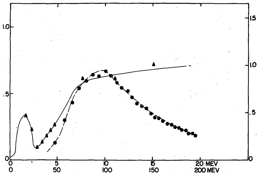
FIG. 2 DEUTERON EXCITATION OF Na^{22} FROM Mg^{24} , Mg^{25} , Mg^{26}
