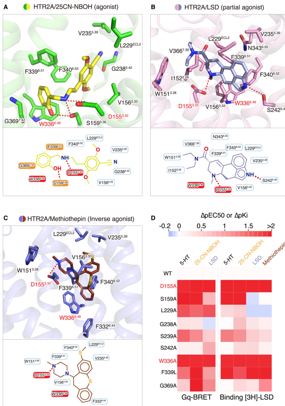
Figure 3. Ligand-Specific Interactions with HTR2A
