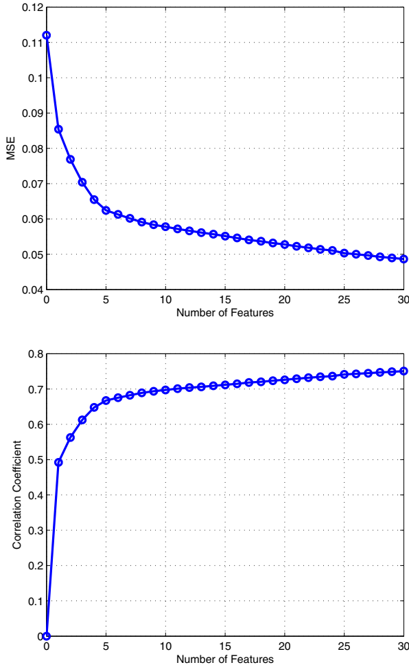
Fig. 8. Performance of the Prediction Model
