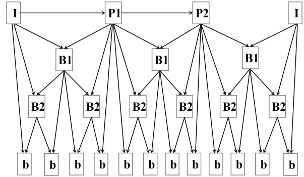
Fig. 2. Hierarchical GOP Structure
