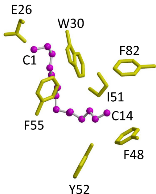
Fig 6. NMR spectroscopy of myristoyl binding site in VILIP-3. Three-dimensional ^{13}\text{C}(\text{F}1) -edited ^{13}\text{C}(\text{F}3) -filtered HMQC NOESY spectra of unlabeled VILIP-3 containing a ^{13}\text{C} -labeled myristoyl group. (A-C) Two-dimensional slices of ^{13}\text{C}(\text{F}1) -edited ( ^{13}\text{C}/\text{F}3 )-filtered HMQC NOESY spectra of ^{13}\text{C} -labeled myristoyl group attached to \text{Ca}^{2+} -free myristoylated VILIP-3 edited at ^{13}\text{C} frequencies 16.89 (A), 34.31 (B) and 37.94 (C) ppm. NOE crosspeaks represent protons of myristate that are less than 5 Å away from aliphatic and aromatic resonances of the \text{Ca}^{2+} -free protein (marked by residue labels). Schematic view of protein contacts along fatty acyl chain (D) and same view rotated by 180^\circ (E). Side-chain atoms of hydrophobic residues near fatty acyl chain are highlighted yellow.
