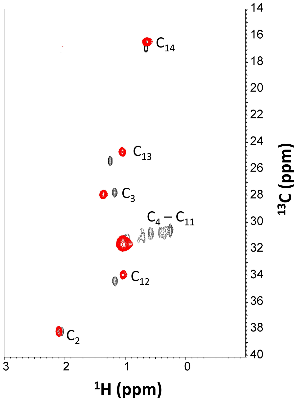
Fig 7. \text{Ca}^{2+} -induced extrusion of myristate. Overlay of two dimensional ^1\text{H} - ^{13}\text{C} HMQC NMR spectra of the ^{13}\text{C} -labeled myristoyl group attached to unlabeled \text{Ca}^{2+} -free VILIP-3 (black peaks) and \text{Ca}^{2+} -bound VILIP-3 (red peaks). The spectral changes reflect \text{Ca}^{2+} -induced environmental changes around the myristoyl group, indicative of \text{Ca}^{2+} -induced extrusion of the myristate. Chemical shift assignments are provided in Table 3.
