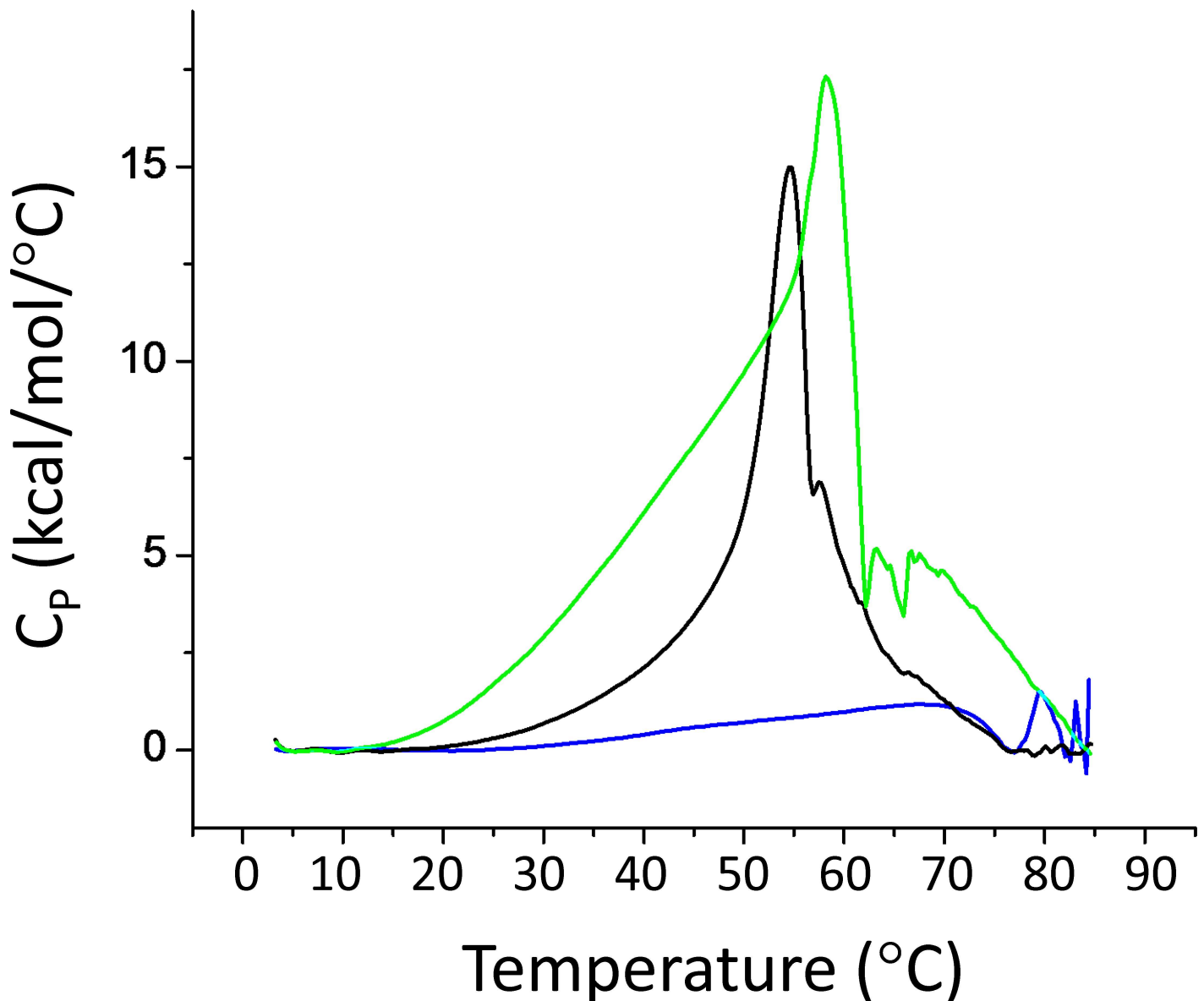
Fig 3. Folding stability of VILIP-3. Representative DSC thermograms for \text{Ca}^{2+} -free VILIP-3 in both unmyristoylated (black) and myristoylated (green) states. The protein unfolding temperatures ( T_M ) determined from the thermograms are listed in Table 1. The T_M for \text{Ca}^{2+} -saturated myristoylated VILIP-3 could not be accurately measured due to complications caused by \text{Ca}^{2+} -induced protein aggregation (see blue trace).
