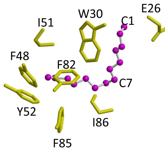
Fig 6. NMR spectroscopy of myristoyl binding site in VILIP-3. Three-dimensional ^{13}\text{C}(\text{F}1) -edited ^{13}\text{C}(\text{F}3) -filtered HMQC NOESY spectra of unlabeled VILIP-3 containing a ^{13}\text{C} -labeled myristoyl group. (A-C) Two-dimensional slices of ^{13}\text{C}(\text{F}1) -edited ( ^{13}\text{C}/\text{F}3 )-filtered HMQC NOESY spectra of ^{13}\text{C} -labeled myristoyl group attached to \text{Ca}^{2+} -free myristoylated VILIP-3 edited at ^{13}\text{C} frequencies 16.89 (A), 34.31 (B) and 37.94 (C) ppm. NOE crosspeaks represent protons of myristate that are less than 5 Å away from aliphatic and aromatic resonances of the \text{Ca}^{2+} -free protein (marked by residue labels). Schematic view of protein contacts along fatty acyl chain (D) and same view rotated by 180^\circ (E). Side-chain atoms of hydrophobic residues near fatty acyl chain are highlighted yellow.
