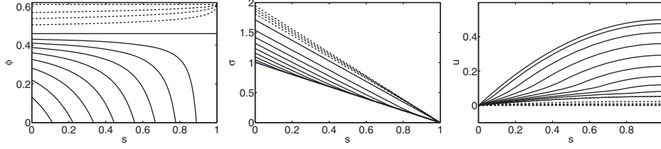
FIG. 3. Plots of the solutions to (2.3) for angle = 30^\circ . The x-axis is s . Different curves refer to different initial data \phi_0 with solid line representing \phi_0 < \phi_{crit} and dashed line \phi_0 > \phi_{crit} . Left: particle volume fraction \tilde{\phi} ; middle: shear stress \tilde{\sigma} ; right: suspension velocity \tilde{u} .
