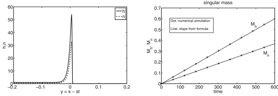
FIG. 10. Simulation of (2.8) using the upwind scheme with initial data (4.25) using a moving mesh y = x - st with s = 0.0222 calculated from (4.24). Left: the profiles of h and n at time t = 600 (corresponding to 0.2 min). Right: the plots of singular mass versus time. The dots are numerical results and the solid lines are calculated by (4.22). Here \Delta y = 1e-3 , \Delta t is chosen adaptively to satisfy the CFL condition.
