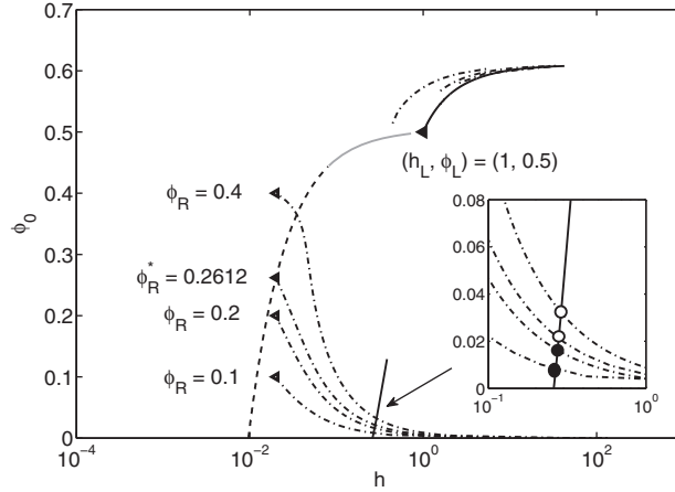
FIG. 13. The Hugoniot loci for left state (h_L, \phi_L) = (1, 0.5) and right states with h_R = 0.02 and \phi_R = \{0.4, 0.2612, 0.2, 0.1\} . The black and gray curves represent admissible 1- and 2- shocks for the left state, and the dashed curve represents an over-compressive shock connecting to the left state. Dashed dots denote an admissible 2-shock connecting to the right states. Here the angle \alpha = 30^\circ .
