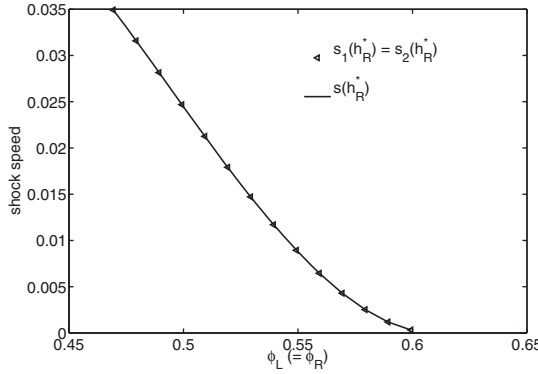
FIG. 11. Comparison of the double shock speeds with the singular shock speed for the left state ( h_L = 1, \phi_L ) with \phi_L changing in (\phi_{crit}, \phi_{max}) and the right state ( h_R^*, \phi_R = \phi_L ). The double shock speeds s_1 (which automatically equals s_2 ) is calculated using (4.31), and the singular shock speed s is obtained using (4.24).
