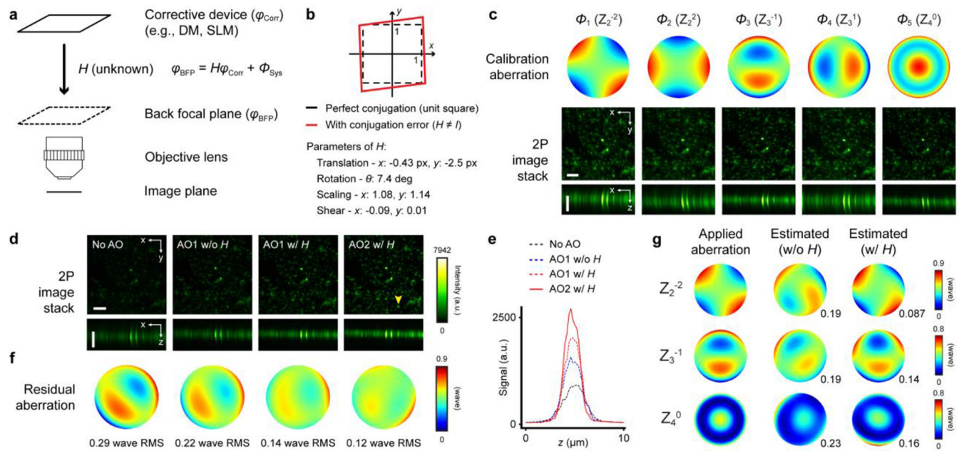
Figure 3. NeAT corrects for conjugation errors in a commercial microscope.
