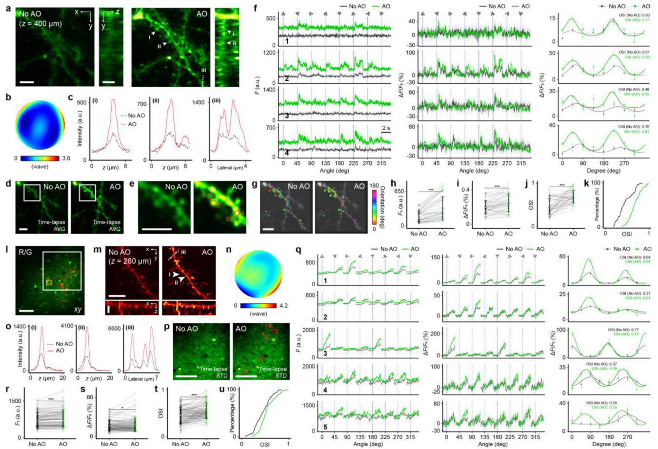
Figure 5. Real-time aberration correction by NeAT for in vivo glutamate and calcium imaging. (a) Lateral ( xy ) and axial ( yz ) MIPs of input stacks to NeAT ("No AO") and stacks acquired after aberration correction by NeAT ("AO") of dendrites expressing iGluSnFR3 at 400 \mu\text{m} depth in mouse V1. (b) Estimated aberration by NeAT. (c) Axial profiles of spines indicated by arrowheads and lateral profiles along dashed line in (a) . (d) Averages of time-lapse xy images of dendrites measured without and with AO. (e) Zoomed-in views of structures in box in (d) . (f) Trial-averaged signal traces ( F ), glutamate transient traces ( \Delta F/F_0 ), orientation tuning curves and OSI values of 4 ROIs (1-4 in (e) ). Shade and error bars: s.e.m. (g) OS spines in (d) color-coded by their preferred orientations measured without and with AO. (h-k) Comparisons of basal fluorescence ( F_0 ; (h) ), glutamate transient ( \Delta F/F_0 ; (i) ), OSIs ( (j,k) ) of 52 OS spines out of 86 total spines before and after AO correction. Two-sided paired t-test ( (h-j) ), p < 0.001 . Kolmogorov-Smirnov test ( (k) ), p < 0.001 . (l) Superimposed xy images of sparse tdTomato-expressing neurons (1000-nm excitation) and dense GCaMP6s-expressing neurons (920-nm excitation) at 280 \mu\text{m} depth. (m) Lateral ( xy ) and axial ( xz ) MIPs of dendrites (yellow box in (l) ) measured without ("No AO", input to NeAT) and with AO. (n) Estimated aberration by NeAT. (o) Axial profiles for spines indicated by arrowheads and lateral profiles along dashed line in (m) . (p) Standard deviation of time-lapse images of GCaMP6s-expressing neurons in white box in (l) , acquired without and with AO. (q) Trial-averaged signal traces ( F ), calcium transient traces ( \Delta F/F_0 ), orientation tuning curves, and OSI values of 5 ROIs (1-5 in (p) ).
