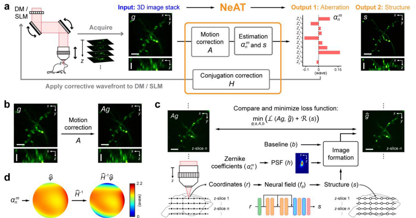
Figure 1. NeAT estimates aberration and recovers structure from a 3D input image stack.
