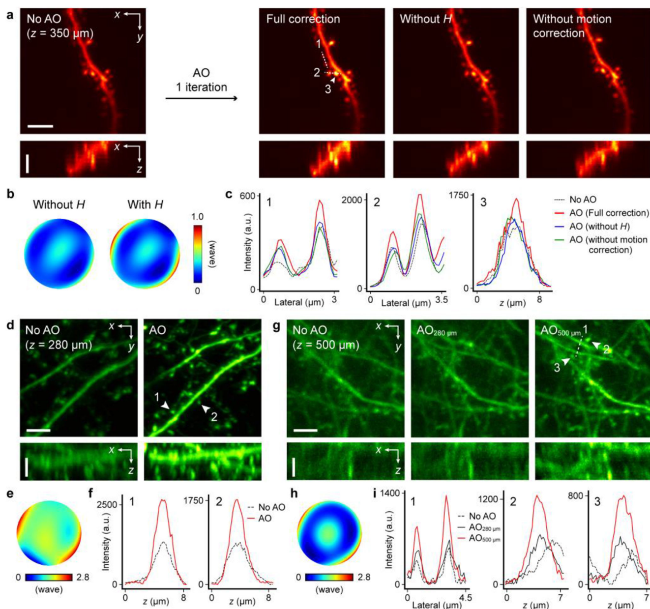
Figure 4. Real-time aberration correction by NeAT for in vivo structural imaging.
