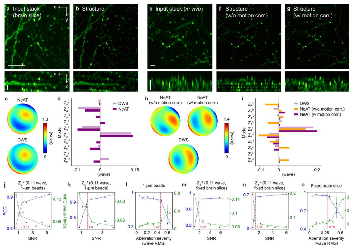
Figure 2. Performance characterization with direct wavefront sensing (DWS) AO in a custom-built 2P microscope.
