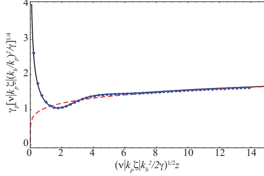
FIG. 2. (Color online) Normalized phase velocity of accelerating wakefield \gamma_p[\nu(k_b/k_p)^2|\hat{\zeta}|/\gamma]^{1/4} vs. normalized propagation distance (\nu|\hat{\zeta}|)^{1/2}\hat{z} in the long-beam regime: solid (black) curve is the series solution Eq. (12), dashed (red) curve is the asymptotic solution Eq. (14), and dots (blue) are from the numerical solution of the envelope equation Eq. (5).
