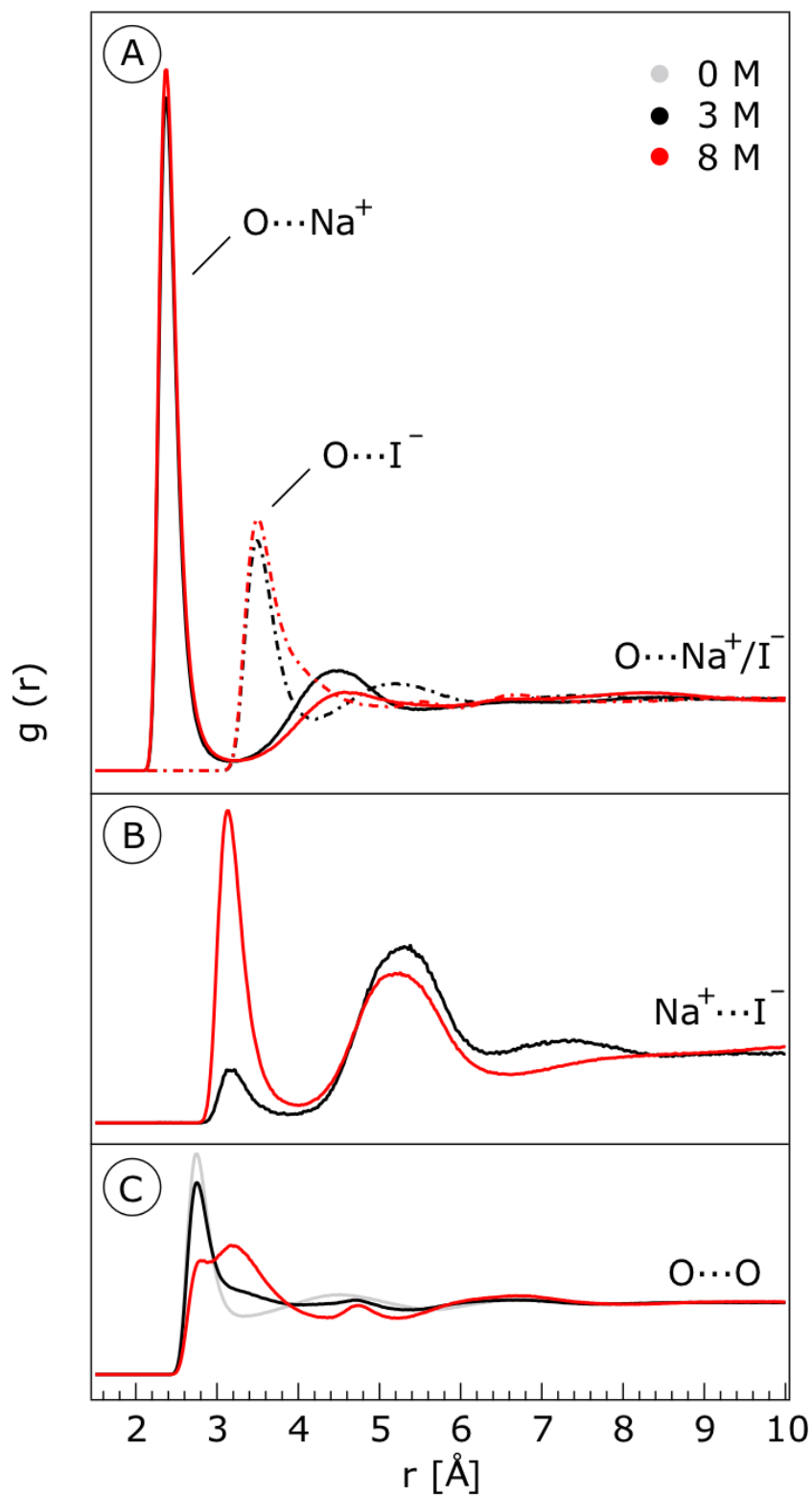
Figure 8 Radial distribution functions for (A) water \text{O}\cdots\text{Na}^+ (solid lines) and water \text{O}\cdots\text{I}^- (dashed-lines) and (B) \text{Na}^+\cdots\text{I}^- in the 3 M and 8 M aqueous solutions of NaI. (C) Radial distribution functions for \text{O}\cdots\text{O} for neat water (labelled 0 M), 3 M and 8 M aqueous solutions of NaI.
