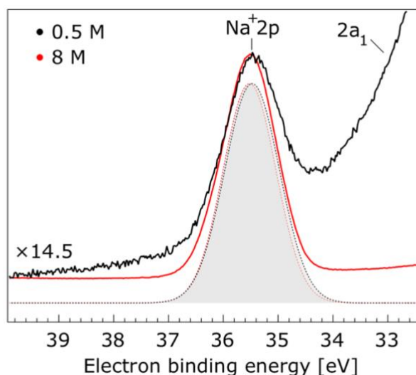
Figure 2 Enlarged view of the \text{Na}^+ 2p and water 2a_1 photoelectron spectra of 0.5 M (black) and 8.0 M (red) NaI (aq) solutions measured at a 198 eV photon energy. The intensity of the 0.5 M concentration spectrum was multiplied by 14.5 to yield the same peak height as that observed from the 8.0 M solution. Gaussian fits of the \text{Na}^+ 2p peak are presented (the fits in black and red correspond to the 0.5 M and 8.0 M solutions, respectively). Spectral contributions primarily associated with water 2a_1 ionization have been subtracted.
