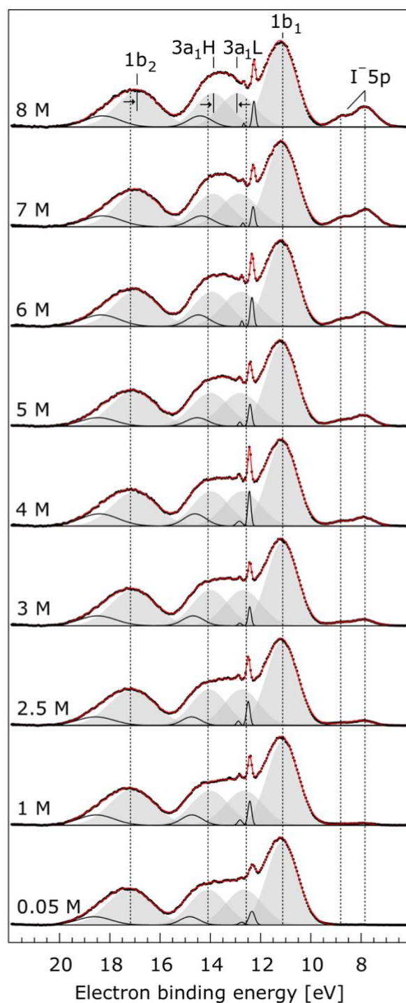
Figure 5 Valence photoelectron spectra from NaI aqueous solutions as a function of concentration, 0.05 M to 8.0 M. The high energy resolution spectra were recorded at the U41 beamline with a photon energy of 180 eV. Intensities are displayed to yield the same liquid water 1b_1 peak heights for each solution. Peaks in grey are the Gaussian fits representing the photoelectron contributions primarily due to ionization of the four liquid water valence orbitals. Solid black lines are Gaussian fits of gas-phase water signal contributions. For the lowest concentration, the fit parameters previously reported for water 32 were used. For the higher concentrations, the energetic positions and widths of all peaks were allowed to vary. Both 3a_1 Gaussian fit component peaks ( 3a_1 L and 3a_1 H , see the main body of the text for details) are constrained so that they exhibit similar widths and heights in each spectrum.
