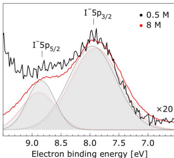
Figure 4 Enlarged view of the \Gamma 5p 3/2 and \Gamma 5p 1/2 photoelectron spectra of 0.05 M (black) and 8.0 M (red) NaI (aq) solutions measured at a 198 eV photon energy. The intensity of the 0.5 M concentration spectrum was multiplied by a factor of 20 to yield the same peak heights as those observed from the 8.0 M solution. Gaussian fits of the \Gamma 5p 3/2 and water \Gamma 5p 1/2 components are presented (the fits in black and red correspond to the 0.5 M and 8.0 M solutions, respectively).
