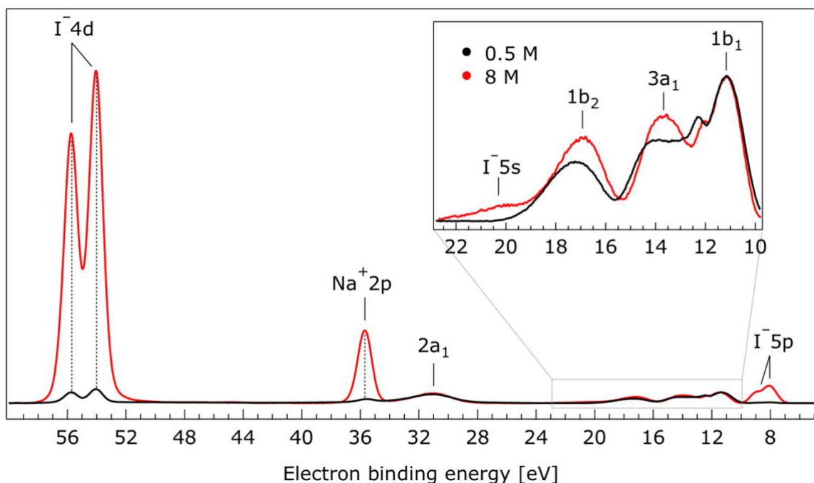
Figure 7 Valence photoelectron spectra of 0.5 M (black) and 8.0 M (red) NaI (aq) measured at a 650.0 eV photon energy. Inset: Enlarged region associated with the outer-valence spectrum.
