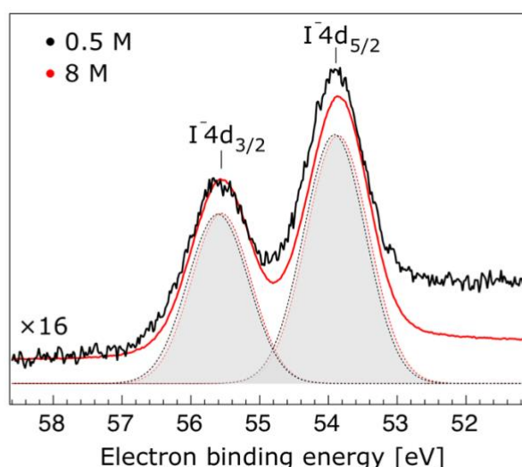
Figure 3 Enlarged view of the \text{I}^- 4d_{5/2} and \text{I}^- 4d_{3/2} photoelectron spectra of 0.05 M (black) and 8.0 M (red) NaI (aq) solutions measured at a 198 eV photon energy. The intensity of the 0.5 M concentration spectrum was multiplied by 16 to yield the same peak heights as those observed from the 8.0 M solution. Gaussian fits of the \text{I}^- 4d_{5/2} and water \text{I}^- 4d_{3/2} components are presented (the fits in black and red correspond to the 0.5 M and 8.0 M
