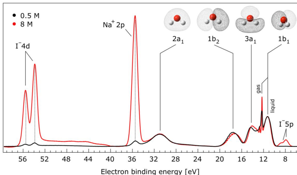
Figure 1 Valence photoelectron spectra of 0.5 M (black) and 8.0 M (red) NaI (aq) measured at a 198.0 eV photon energy at the U49 beamline. A linear background was subtracted from both spectra in order to account for the contributions of the inelastically scattered electrons. Both spectra appear to be closely energetically aligned at the \text{Na}^+ 2p and \text{I}^- 4d peaks after shifting the peak of the liquid water 1b_1 peaks to 11.16 eV, as indicated by dashed lines. Small plateau features in the 41-52 eV BE region for the 8 M solution can be assigned to energy loss processes where \text{Na}^+ 2p photoelectrons excited quasi-optical transitions of water. 112 Schematics of the valence molecular orbitals of water are reprinted from ref. 139 in the top right of the figure.
