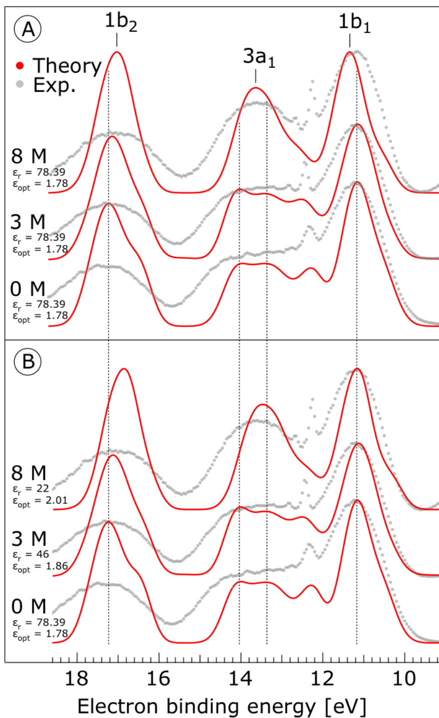
Figure 9 Theoretical photoemission spectra. (A) Simulations for water heptamer clusters containing one \text{Na}^+ and one \text{I}^- ion embedded in a polarizable continuum having a permittivity, \epsilon_r , of 78.39 (which corresponds to pure water) and \epsilon_{\text{opt}} = 1.78 . (B) simulations for the same water clusters embedded in a polarizable continuum having a permittivity \epsilon_r = 46 and \epsilon_{\text{opt}} = 1.86 for the 3 M NaI, and \epsilon_r = 22 and \epsilon_{\text{opt}} = 2.01 for the 8 M NaI solution. Data for water (labelled '0 M') corresponds to water heptamers embedded in a polarizable continuum and having a permittivity of 78.39 in both (A) and (B). Experimental spectra are aligned at the water 1b_1 peak (11.16 eV BE). All theoretical spectra are shifted to lower energies by 0.3 eV, so that the spectra representing pure water are aligned at the known 1b_1 BE as well.
