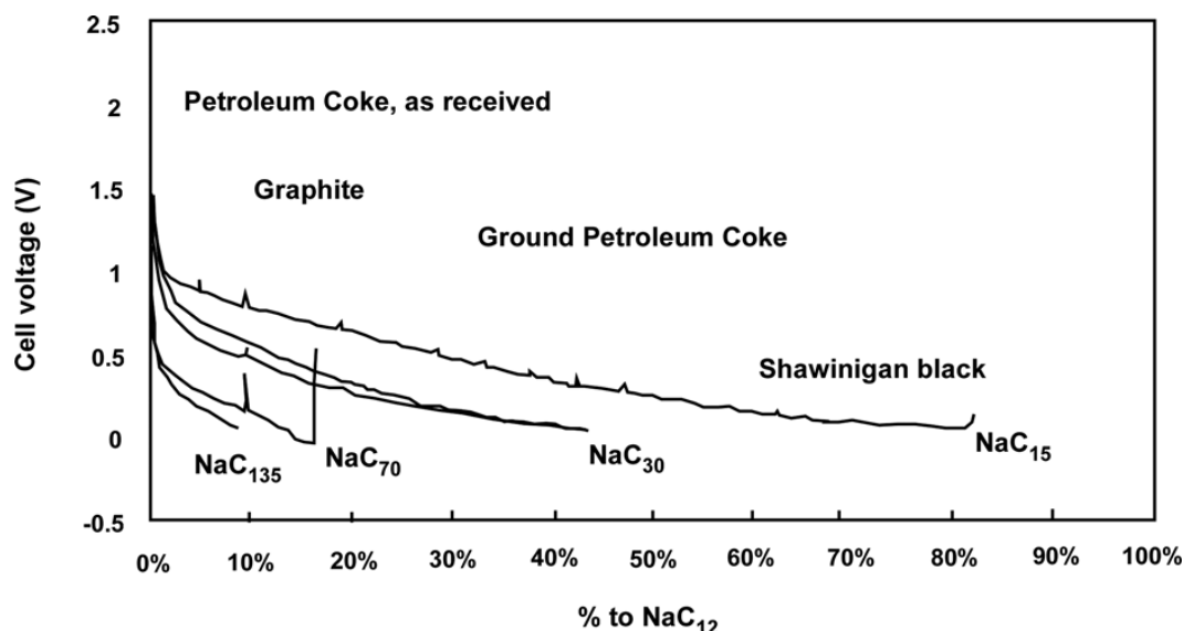
Figure 1-23. Discharge curves ( 50 \text{ mA cm}^{-2} ) of \text{Na/P(EO)}_8\text{NaCF}_3\text{SO}_3/\text{C} cells heated to 86^\circ\text{C} . The spikes in the profiles are due to periodic current interrupts to assess the cell polarization. 180
