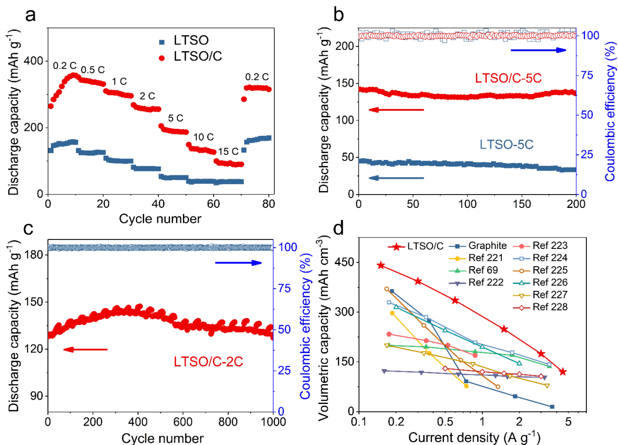
Figure 4-10. Galvanostatic cycling of half-cells: a) rate test ( 1\text{ C} = 300\text{ mA g}^{-1} ); b) durability test at 5\text{ C} ; c) long-term cycling test of LTSO/C at 2\text{ C} (low voltage cutoff: 0.1\text{ V} ). d) Comparison between LTSO/C with anode counterparts (graphite, \text{TiO}_2 , LTO) in volumetric capacity-current density plot.
