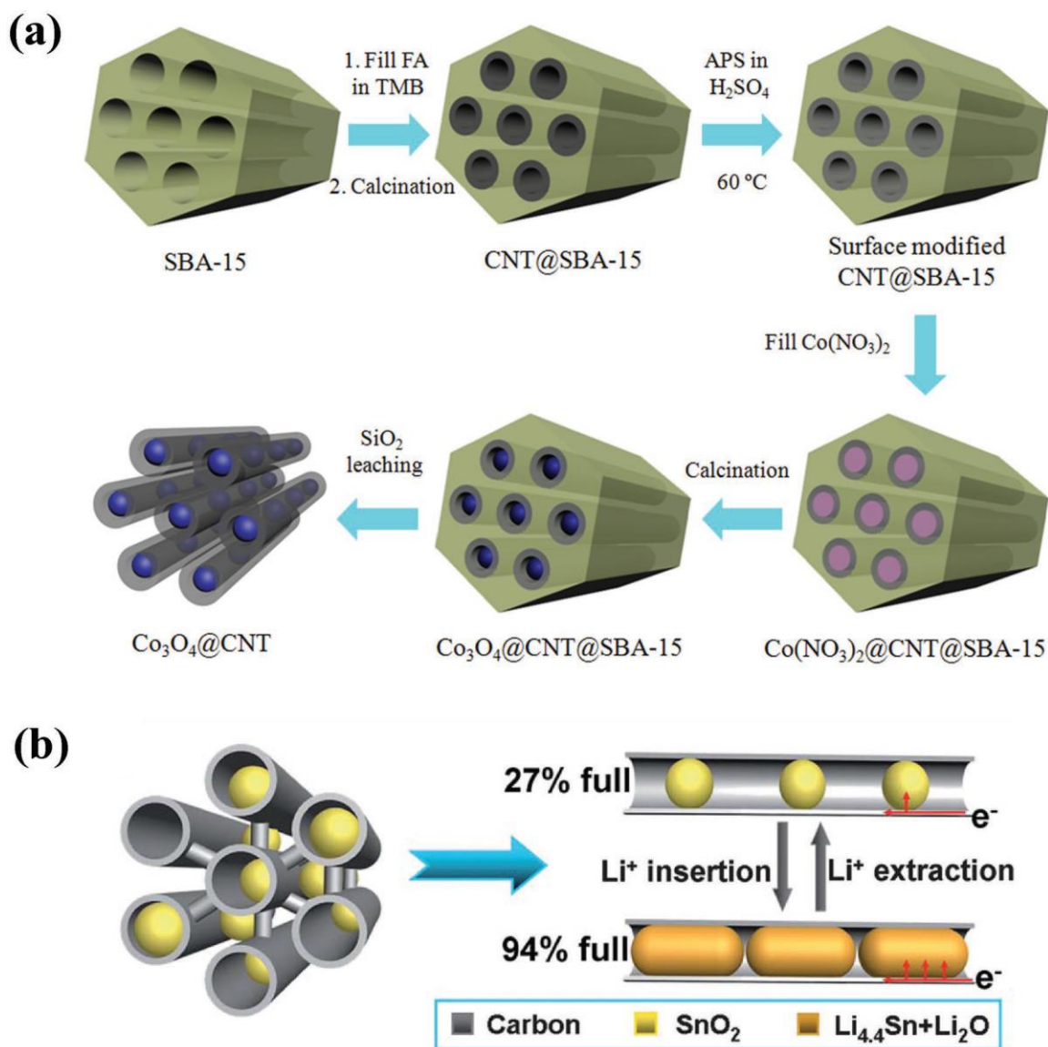
Figure 1-8. a) Schematic illustration of the formation process of mesoporous peapod-like \text{Co}_3\text{O}_4 @carbon nanotube arrays. b) Schematic illustration of volume change during \text{Li}^+ insertion/extraction processes in \text{SnO}_2 /CMK-5 composite. 95
