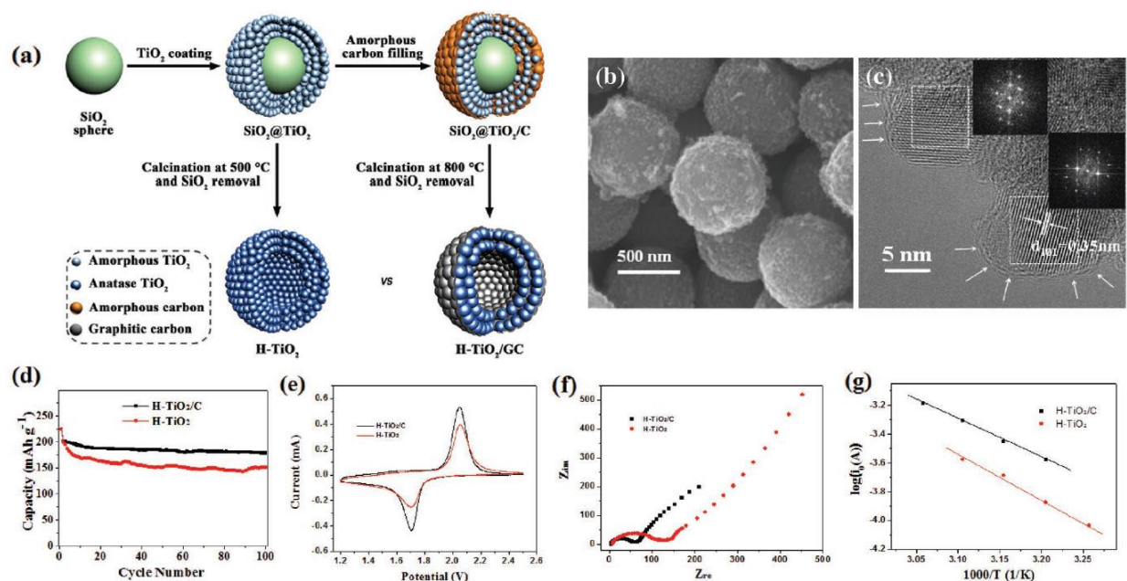
Figure 1-9. a) Schematic illustration of the formation of conformal graphitic carbon coating of mesoporous hollow TiO 2 (Denoted as H-TiO 2 /GC) spheres. b) SEM and c) TEM images of the mesoporous H-TiO 2 /GC hollow sphere d) Cycling performance of H-TiO 2 /GC and H-TiO 2 spheres at a constant current density of 0.1 A g -1 (approximately 0.5 C). Inset images show the structural evolution of H-TiO 2 and H-TiO 2 /GC spheres upon cycling. e) Cyclic voltammetry (CV) curves of H-TiO 2 /GC and H-TiO 2 sphere electrodes with a scanning rate of 0.5 mV s -1 . f) Nyquist plots of H-TiO 2 /GC and H-TiO 2 spheres at room temperature. g) Activation energy and corresponding Arrhenius plots of log i 0 versus 1/T for fresh electrodes of H-TiO 2 /GC and H-TiO 2 spheres collected at 2 V at different temperatures from 35 to 55 °C. 95
