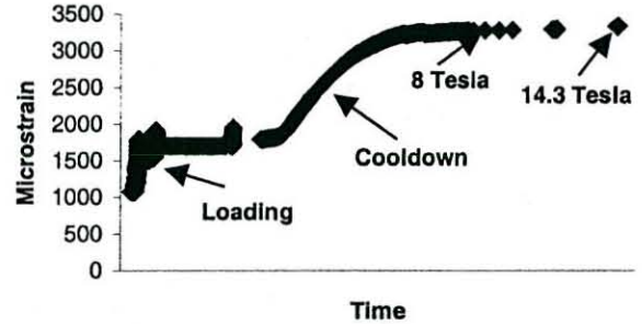
Figure 3: Pre-stress history, from loading through cool-down and magnet excitation for the first cycle.
