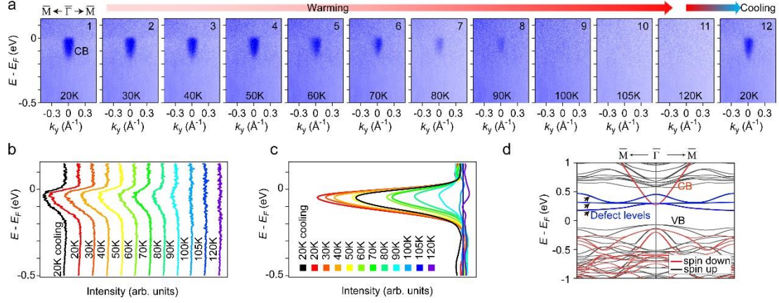
Figure 3. Half-metal driven by ferromagnetism in n -HgCr 2 Se 4 . (a) Evolution of bands along \bar{M}-\bar{\Gamma}-\bar{M} after K dosing at different temperatures. They are normalized in the same way as in Figure 2(g-h). (b) Extracted temperature dependent EDCs from (a) with a momentum integration of \pm 0.025 \text{ \AA}^{-1} . (c) Overlaid temperature dependent EDCs from (b). They are divided by the EDC at the temperature of 105K. (d) The spin-resolved band structure from the Hg 15 Cr 32 Se 63 supercell (Hg vacancy level is 1/16 and Se vacancy level is 1/64) which has defect levels from Hg and Se vacancies. The ones labeled by the blue color are mainly from the Se vacancies.
