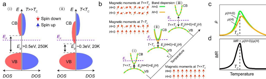
Figure 4. Electronic origin of the HMST and CMR in n -HgCr 2 Se 4 . (a) Schematic of the electronic origin of the HMST. (i) T \gg T_c , the CB and VB have no spin related splitting. The band gap ( E_g ) is > 0.5 \text{ eV} at 250K (SI4-5). (ii) T \ll T_c , the CB splits and crosses E_F while the VB has minor changes (SI4-5). The band gap narrows to \sim 0.3 \text{ eV} at 20K. (b) Schematic of the electronic origin of the CMR. (i-iii) Temperature dependent band structure with and without magnetic field at T \ll T_c (i), T \sim T_c (ii) and T \gg T_c (iii). Inset: Schematic of the alignment of the magnetic moments by magnetic field across T_c . (c) Schematic of the temperature dependent resistivity curve ( \rho - T ) of the HMST according to the electronic evolution in (b). (d)
