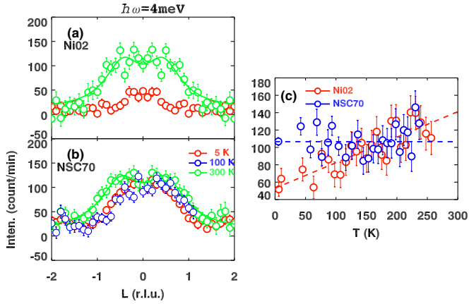
FIG. 4. Inelastic neutron scattering measurements on (a) NiO2 and (b) NSC70 samples along (0.5, 0, L) at energy transfer \hbar\omega = 4 meV, performed on BT7. The solid lines are fits to the two symmetric Lorentzian peaked at L = \pm 0.5 . The intensities at (0.5, 0, 0.5) vs. T for both samples are plotted in (c). The dashed lines are guides to the eye. The error bars represent statistical error.
