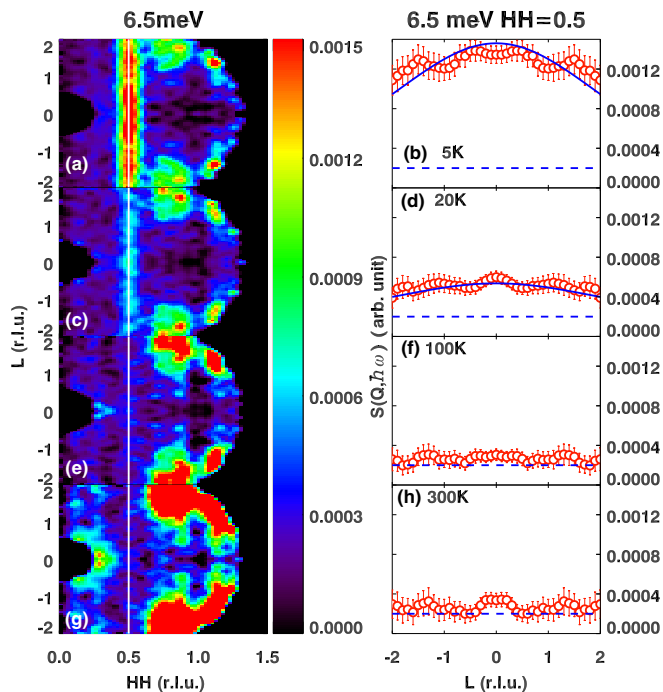
FIG. 2. Inelastic neutron scattering intensity in the (HLL) plane measured on HYSPEC at energy transfer \hbar\omega = 6.5 meV from the SC40 sample. Left column are 2D intensity slices, and right column are linear cuts along (0.5, 0.5, L) , obtained at (a) and (b): 5 K; (c) and (d) 20 K; (e) and (f) 100 K; and (g) and (h) 300 K. The q -width of the linear cuts is 0.05 r.l.u. along [110] direction. The white line along (0.5, 0.5, L) in the left panels shows where the L cuts in the right column were taken. The dashed lines in right panels are the estimated background obtained from fitting around (0.65, 0.65, 0) . The blue solid lines in (b) and (d) are magnetic form factors for a \text{Fe}^{2+} ion scaled to the data average. All slices were taken with an energy width of 2 meV. The error bars represent statistical error.
