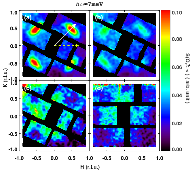
FIG. 1. Inelastic neutron scattering measurements in the (HK0) plane measured on SEQUOIA at energy transfers \hbar\omega = 7 meV from (a)–(c) SC40 and (d) Ni10 samples. The samples temperatures are (a) 5 K, (b) 20 K, (c) 200 K, and (d) 5 K. All slices were taken with an energy width of 2 meV. Intensity scale is the same in (a) to (c); data in (d) have been scaled to be directly comparable. Black regions of each panel represent gaps in the detector array.
