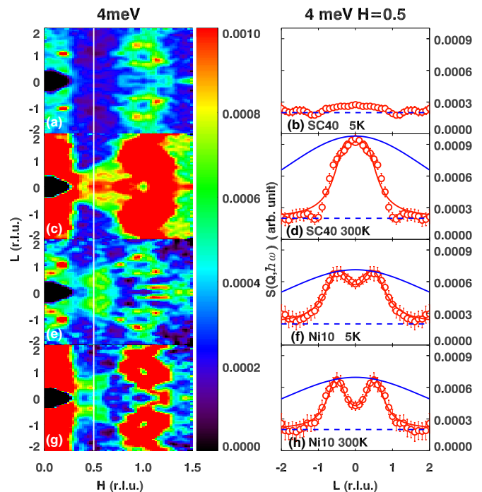
FIG. 3. Inelastic neutron scattering intensities in the (HOL) plane measured on HYSPEC at energy transfer \hbar\omega = 4 meV on the SC40 and Ni10 samples. The intensities are scaled by the sample mass for better comparison. Left column are 2D intensity slices, and right column are linear intensity cuts along (0.5, 0, L) . The q width of the linear cuts is 0.05 r.l.u. along [100] direction. The panels are (a) and (b): SC40 at 5 K; (c) and (d) SC40 at 300 K; (e) and (f) Ni10 at 5 K; and (g) and (h) Ni10 at 300 K. The white line in the left panels at H = 0.5 shows where the L cuts in the right column were taken. The dashed lines in right panels are estimated background values obtained from fitting around (0.65, 0, 0) . The blue solid lines in (d), (f), and (h) are magnetic form factors for a \text{Fe}^{2+} ion scaled to the data range, and the red solid lines are fits to the data using two symmetric Lorentzians peaked at L = \pm 0.5 . All slices were taken with an energy width of 2 meV. The error bars represent statistical error.
