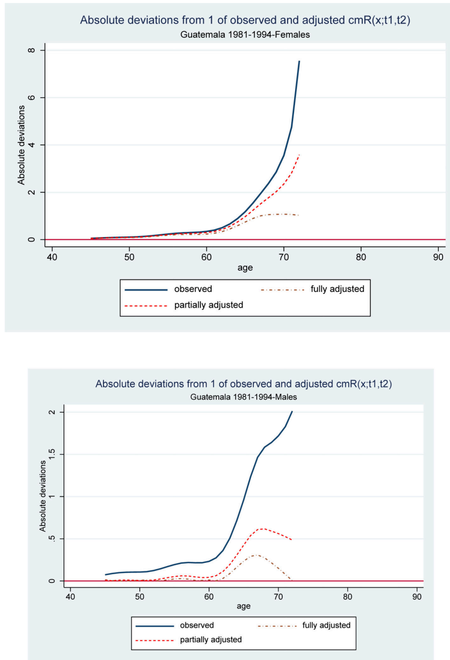
Figure 4. Absolute deviations of observed, partially, and fully adjusted values of cmR_{x,[1981,1994]} from vector of ones, by sex: Guatemala 1981–94. Source: Authors' calculations. Data and code available at https://gitlab.com/csic-echo/lambda-pop
