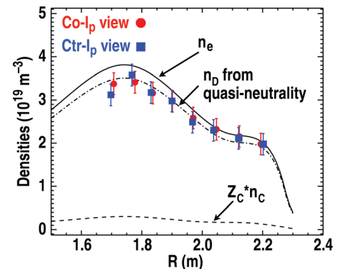
FIG. 10. Density profiles of electrons, thermal deuterium, and fully ionized carbon at the same time as Figs. 8 and 9(a) in the L-mode phase of the discharge.
