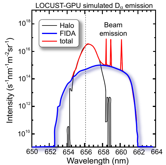
Figure 13. Simulated D_\alpha emission from LOCUST-GPU. FIDA and halo emission result from charge exchange between injected neutrals and, respectively, fast and bulk deuterium ions, while beam emission is produced by the de-excitation of injected neutrals.
