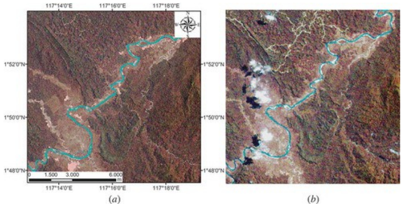
Figure 5. False-colour composite (bands 4, 2, 1) of the image acquired over Berau municipality, Indonesia. (a) 26 August 200; (b) 31 May 2003.
