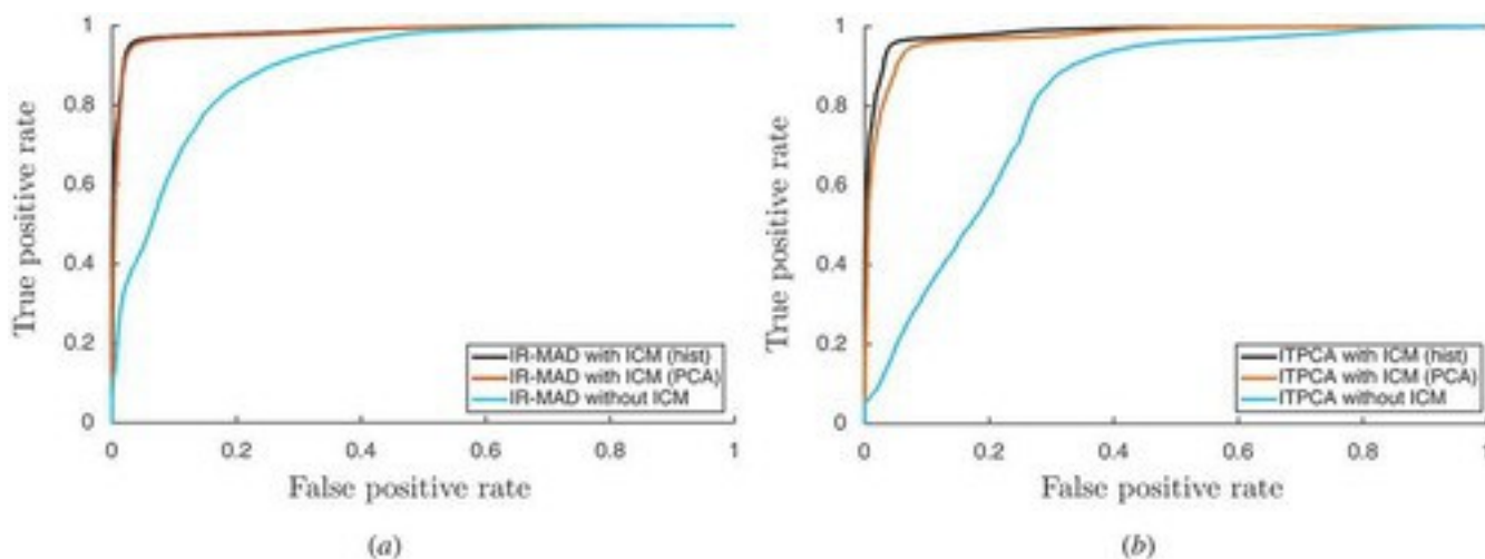
Figure 11. ROC curves computed for the German data set considering the chi-square images obtained by applying (a) IR-MAD, (b) ITPCA.
