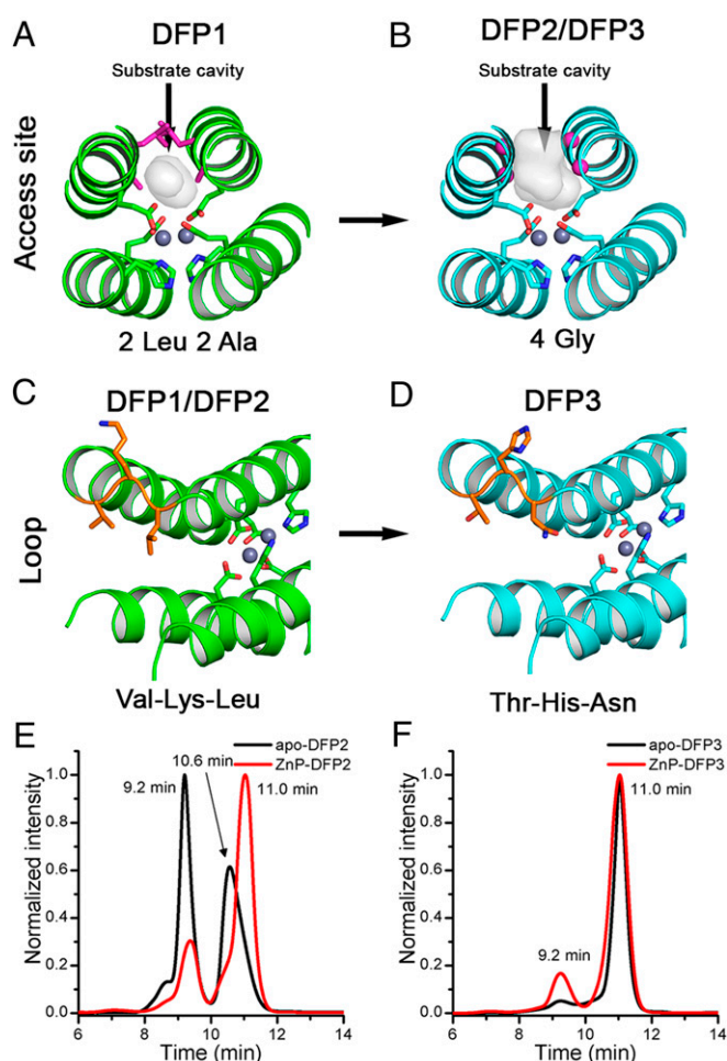
Fig. 3. Engineering functionality in DFP family. The substrate cavity at the dimetal site was broadened mutating the 2 Leu and 2 Ala residues in DFP1 (shown as magenta sticks in A) in 4 Gly residues in DFP2 and DFP3 (shown as magenta spheres in B). To improve the oligomeric behavior, we mutated the Val-Lys-Leu loop in DFP1 and DFP2 (shown as orange sticks in C) in Thr-His-Asn in DFP3 (shown as orange sticks in D). The backbone is shown as green and cyan cartoon before and after the mutations, respectively. The coordinating residues of the dimetal center are shown as sticks, and the metal ions in gray spheres. (E) SEC of apo-DFP2 (in black) and ZnP-DFP2 (in red) at pH 7 (Hepes 50 mM, NaCl 100 mM), followed at 280 nm. (F) SEC of apo-DFP3 (in black) and ZnP-DFP3 (in red) at pH 7 (Hepes 50 mM, NaCl 100 mM), was followed at 280 nm. Retention time peaks at 10.6 min and 11.0 min corresponded to hydrodynamic radii of 27 Å and 21 Å, respectively.
