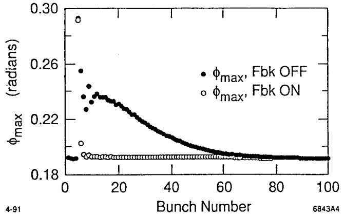
Figure 2. Plot of the maximum bunch offset reached in 3000 turns for the first 100 bunches after the gap, with and without feedback.
