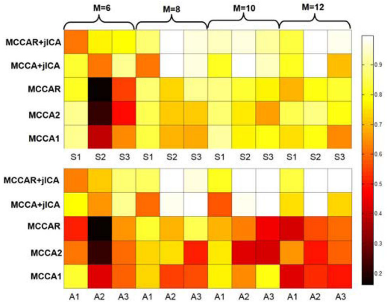
Fig. 5. Performance comparison when using different number of component M for decomposition. True source number = 8, here M varies from 6 to 12. The color of squares represent the correlation between the estimated target IC and the ground truth on either source maps (top) or mixing coefficients (bottom) for different methods. The brighter square color, the higher estimation accuracy. Modality 1, 2, 3 denotes fMRI, dMRI and sMRI respectively. MCCAR +jICA achieves best estimation when M \geq true source number.
