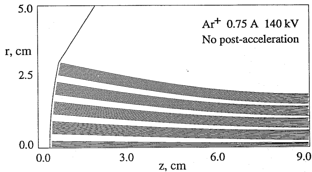
Fig. 5. Beam simulation to check emittance growth from free field energy in merging beams.
