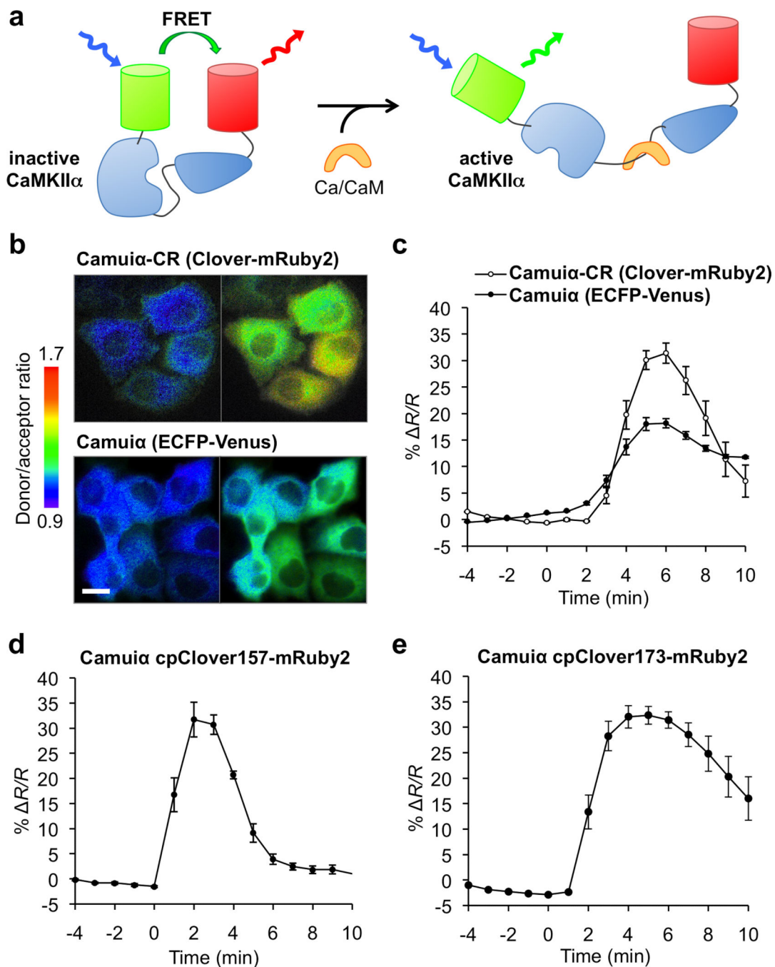
Figure 2. Clover-mRuby2 improves responses versus ECFP-Venus in the CaMKII \alpha reporter Camuia. (a) Organization of Camuia-CR, based on Camuia. (b) Intensity-modulated ratiometric images of HeLa cells expressing Camuia-CR or Camuia before and after addition of 1 \mu M ionomycin at time = 0. Scale bar, 20 \mu m. (c) Mean donor/acceptor emission ratio changes over time. Error bars represent standard error of the mean (s.e.m.). n = 10 cells for Camuia, n = 12 cells for Camuia-CR. Difference in peak emission ratio change is statistically significant ( P = 7.6e-5 ). (d,e) Similar emission ratio responses were obtained with modified
