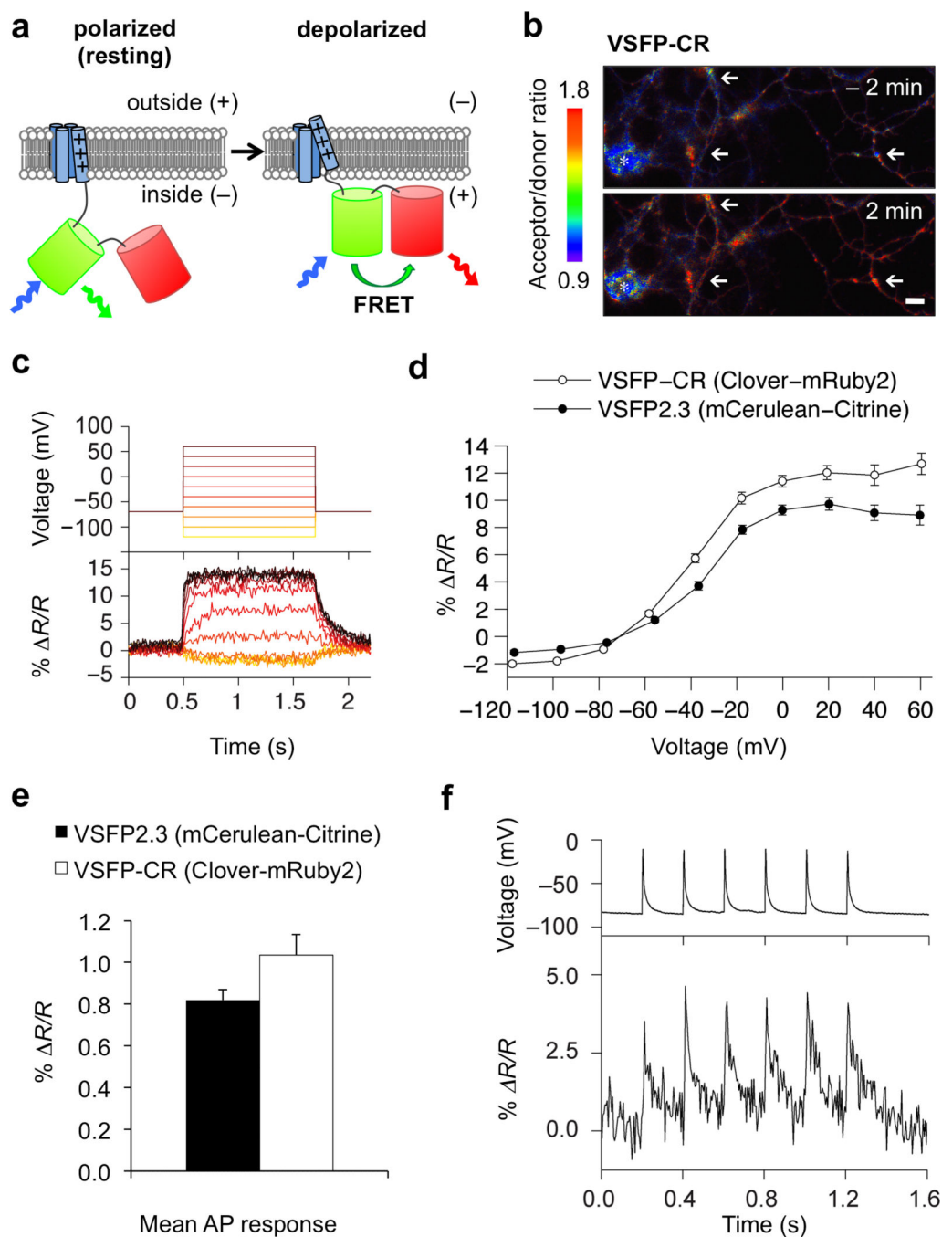
Figure 3. Clover-mRuby2 FRET in voltage sensing. (a) Organization of VSFP-CR, based on VSFP2.3. (b) Ratiometric images of hippocampal neurons expressing VSFP-CR before and after depolarization with 50 mM KCl. Increased acceptor/donor emission was observed at the cell membranes and in neurites (arrows), but not inside the cell body (asterisk). Scale bar, 10 \mu m. (c) For voltage-emission ratio relationships, hippocampal neurons expressing VSFP-CR were subjected to various voltage steps from a resting potential of -70mV by patch-clamping (top panel), and emission ratio changes at each voltage were measured
