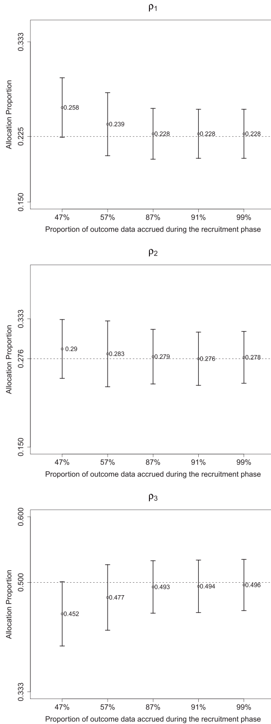
Figure 3 Effect of delayed response on convergence of the compound optimal design (III) to the target allocation \rho = (0.225, 0.275, 0.500) . Displayed are means \pm SD.
